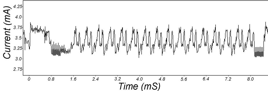
Figure 2.4: SPA Trace of Entire DES Algorithm [4]
