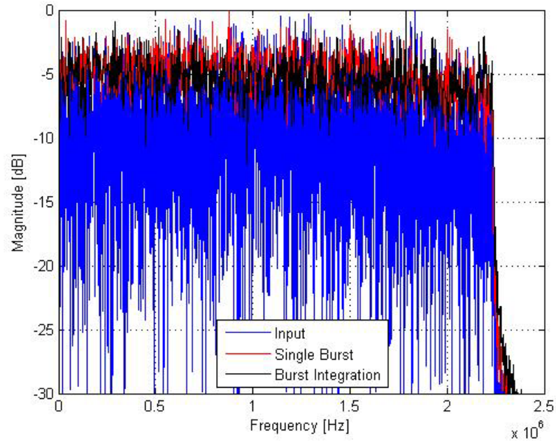
Figure 4.29 Average PSD responses for 802.16e WiMAX data-only burst.
