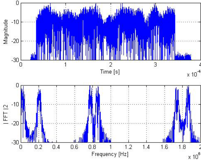
Figure 4.15. Time and PSD responses for single 802.16e WiMAX range-only burst.
