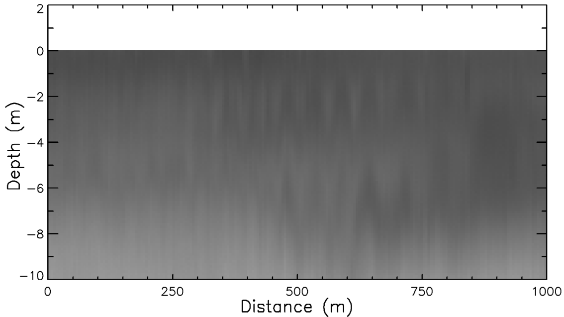
Fig. 1. Lidar return (darker is higher return) as a function of depth and distance along the flight track. Two distinct layers can be seen; both are being perturbed by an internal wave.
