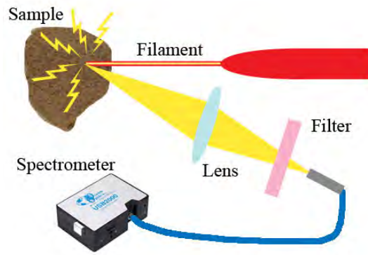
Fig. 7. Experimental setup for measuring spectra from samples ablated with a femtosecond laser filament.
