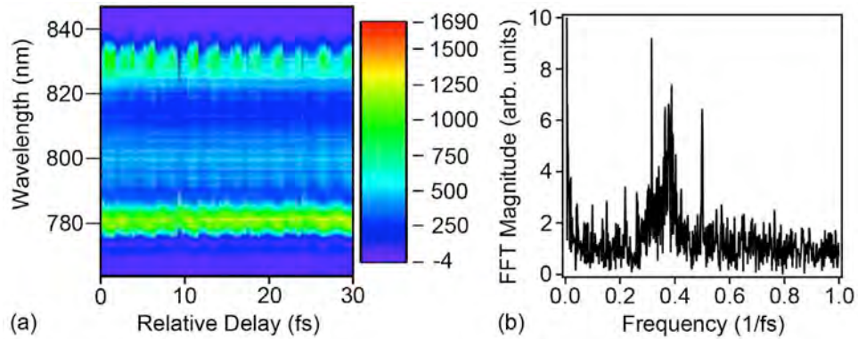
Fig. 3. (a) Raw spectral measurement showing pulse spectrum as a function of relative pulse delay. (b) FFT of (a) showing that the frequency of the oscillations is equal to that of the laser pulse central frequency.
