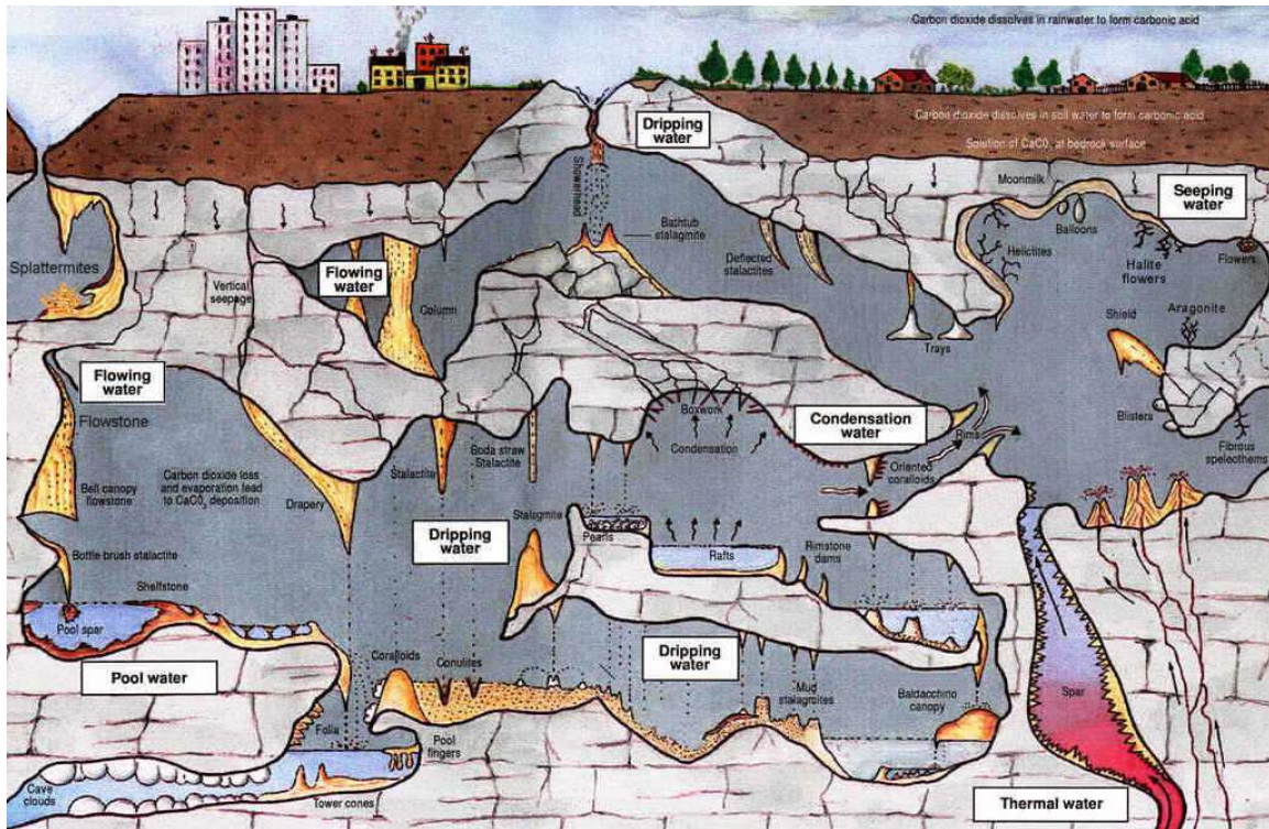
Figure 26: Depiction of the formation of speleothems, through the formation of Carbonic acid and the dissolving of Calcium Carbonate.
