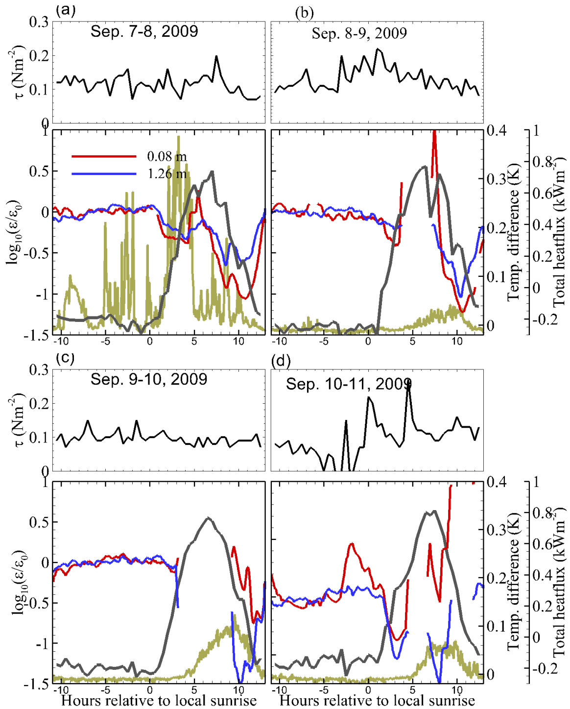
Figure 1. Wind stress, \tau , the ratio of turbulent dissipation rate \epsilon normalized by the averaged dissipation rates from -10 hours to -2 hours, \epsilon_0 , for two depths (0.08 m (red) and 1.26 m (blue)), the total heat flux (black lines), and the temperature difference between 3 m and 15 m (green lines) are plotted versus time in hours relative to the local sunrise for four periods: (a) 7-8 September 2009, (b) 8-9 September 2009, (c) 9-10 September 2009, and (d) 10-11 September 2009.
