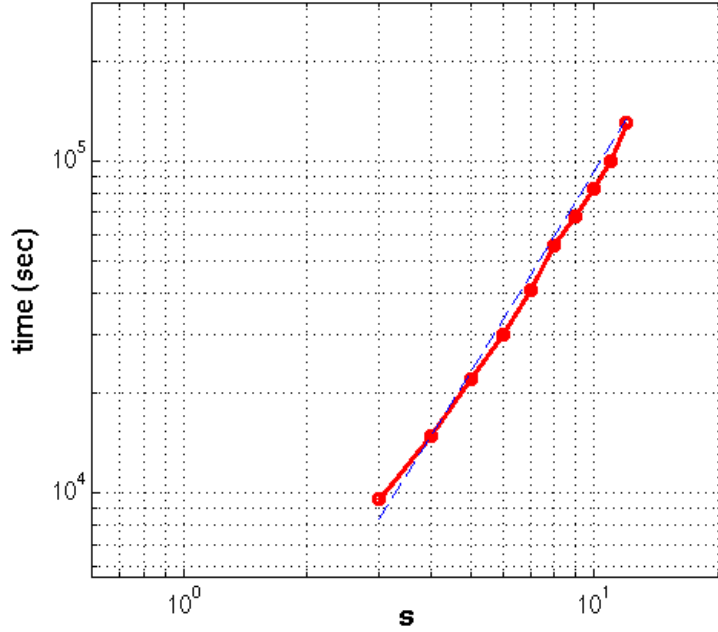
Figure 4-1: Computational time (sec) for the lid-driven cavity flow described in Chapter 5, using different number of modes (red curve). The blue line indicates the linear 'best fit' in the log-log plot and it has an inclination equal to 1.986 (2 is the theoretical prediction).
