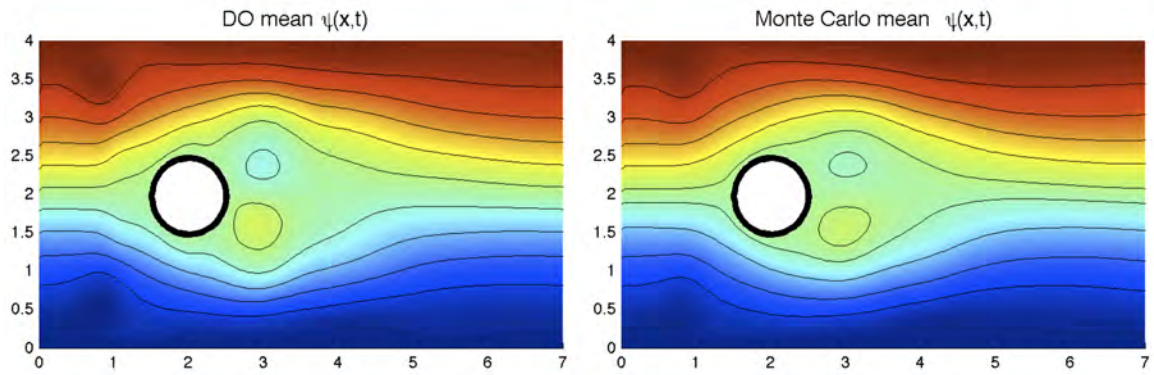
Figure 5-22: Mean velocity field (streamfunction) computed using the DO field equations ( s = 5 ) and Monte-Carlo method (500 samples) at t = 1 .
