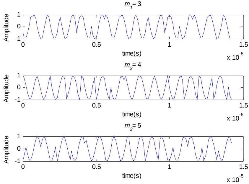
Figure 59. Robust symmetrical residue-P4 signal without noise for m_1 = 3 , m_2 = 4 , and m_3 = 5 with \hat{M}_{RSNS} = 43 , A = 1 , f_c = 1 MHz, f_s = 9 MHz, c_{pp} = 1 , and t'_b = 0.33 \mu s .
