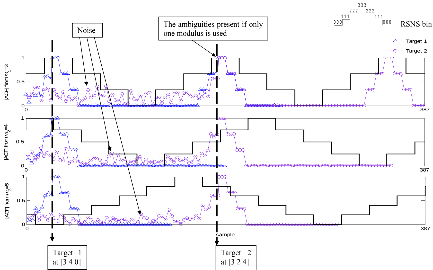
Figure 62. Target detection for SNR = 30 dB showing the range bins for m_1 = 3 , m_2 = 4 , and m_3 = 5 with two targets at 140 m and 1040 m.
