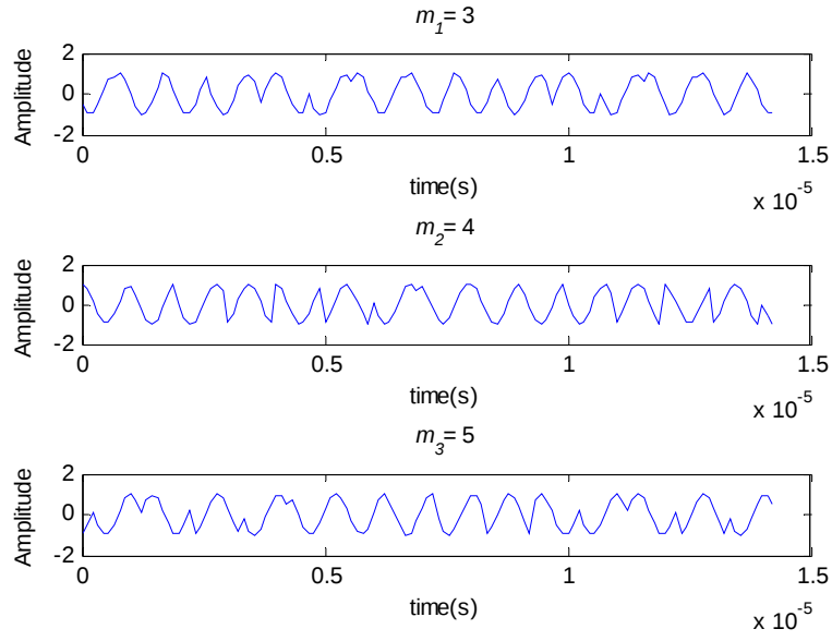
Figure 60. Robust symmetrical residue-P4 signal with SNR = 30 dB for m_1 = 3 , m_2 = 4 , and m_3 = 5 with \hat{M}_{RSNS} = 43 , A = 1 , f_c = 1 MHz, f_s = 9 MHz, c_{pp} = 1 , and t'_b = 0.33 \mu s .
