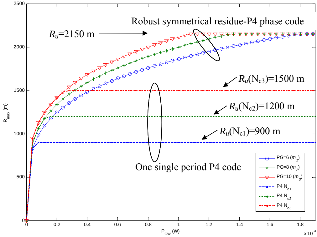
Figure 66. Comparison of the maximum unambiguous range of CW radar system for SNR_{Ro}=13 dB using robust symmetrical residue-P4 code for m_1=3 , m_2=4 , and m_3=5 with the radar using each P4 code individually for the corresponding N_c = N_{c,RSNS}/N .
