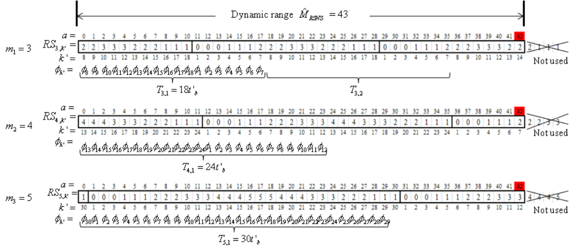
Figure 54. Illustration of transmitted signal using N = 3 robust symmetrical residue-P4 phase code sequences for m_1 = 3 , m_2 = 4 , and m_3 = 5 .
