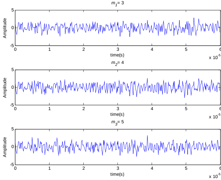
Figure 22. Residue-Frank signal with SNR = 0 dB for m_1 = 3 , m_2 = 4 , and m_3 = 5 with M_{RNS} = 60 , A = 1 , f_c = 1 MHz, f_s = 7 MHz, c_{pp} = 1 , and t_b = 1 \mu s .
