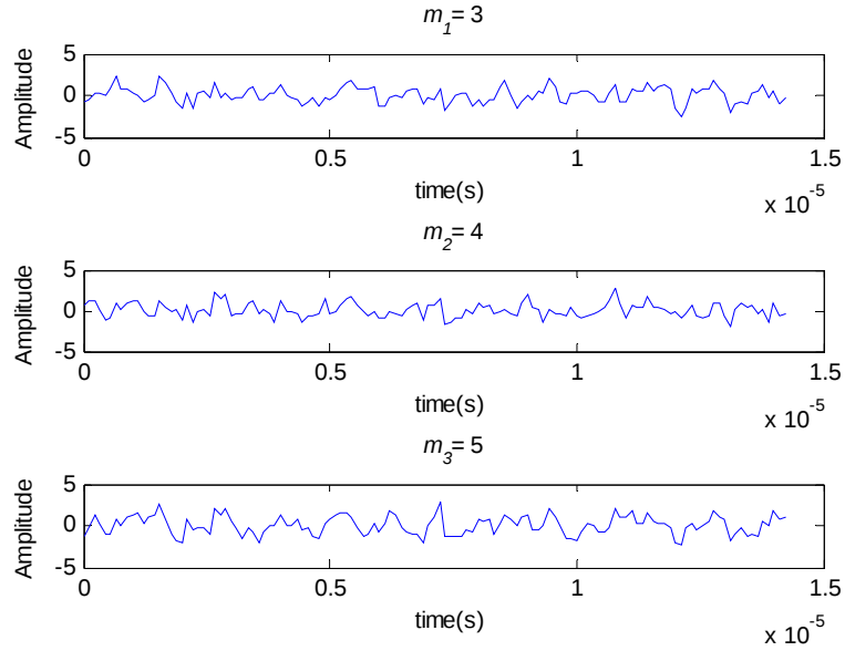
Figure 61. Robust symmetrical residue-P4 signal with SNR = 0 dB for m_1 = 3 , m_2 = 4 , and m_3 = 5 with \hat{M}_{RSNS} = 43 , A = 1 , f_c = 1 MHz, f_s = 9 MHz, c_{pp} = 1 , and t'_b = 0.33 \mu s .
