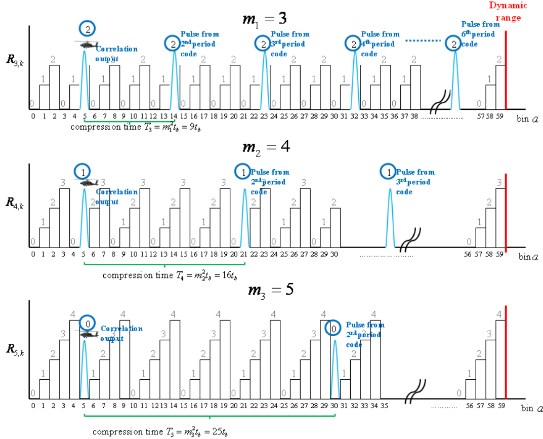
Figure 17. Example of compression output for target detection using N = 3 residue-Frank phase code sequences with m_1 = 3 , m_2 = 4 , and m_3 = 5 .
