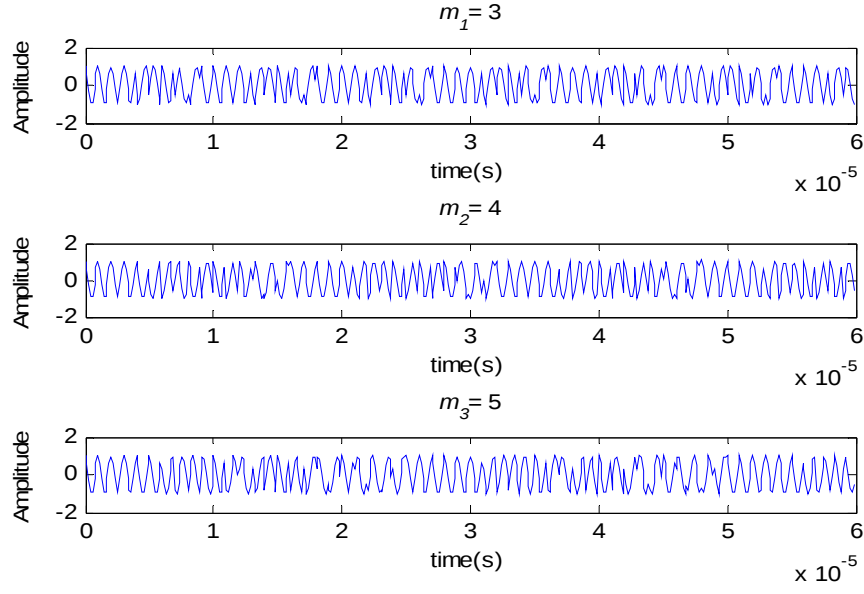
Figure 21. Residue-Frank signal with SNR = 30 dB for m_1 = 3 , m_2 = 4 , and m_3 = 5 with M_{RNS} = 60 , A = 1 , f_c = 1 MHz, f_s = 7 MHz, c_{pp} = 1 , and t_b = 1 \mu s .
