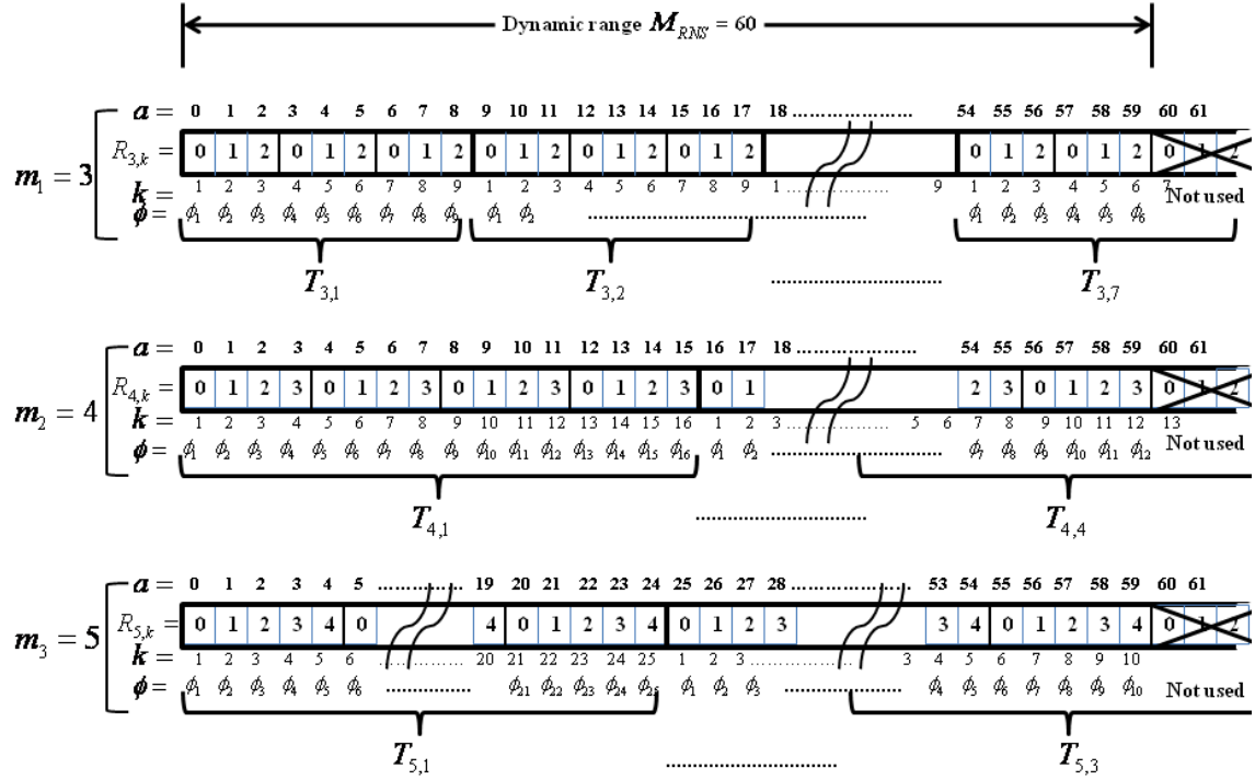
Figure 14. Illustration of transmitted signal using N = 3 residue-Frank phase code sequences for m_1 = 3 , m_2 = 4 , and m_3 = 5 .
