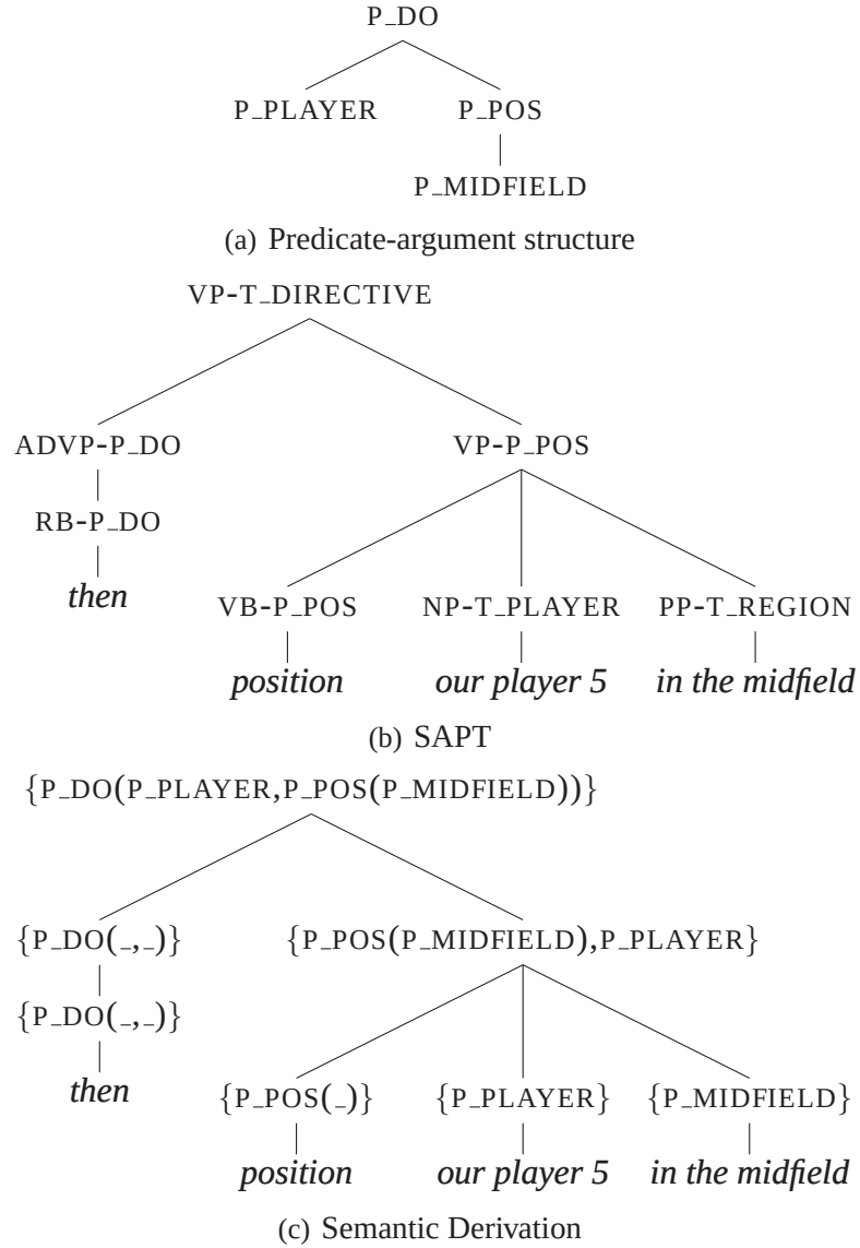
Figure 3.5: (a) The predicate-argument structure, (b) SAPT, and (c) semantic derivation for the directive part of the example in Figure 3.1 (The internal structure of P\_PLAYER in (a) and multi-word leaf nodes in (b) and (c) are omitted for brevity).
