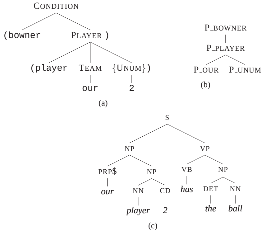
Figure 5.3: Parses for the condition part of the CLANG in Figure 5.2: (a) The parse of the MR (the nodes for parentheses are not separately shown for brevity). (b) The predicate argument structure of (a). (c) The parse of the NL.
