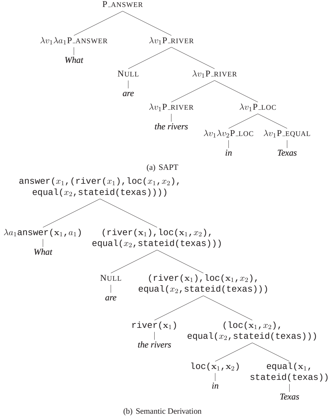
Figure 5.11: Semantic parse for the GEOQUERY example in Fig. 5.8 using the syntactic parse in Fig. 5.10(c).
