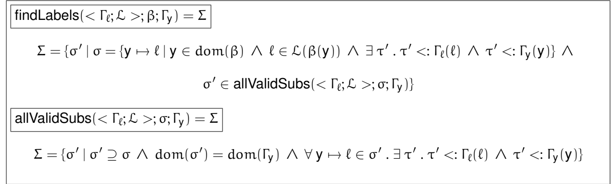
Figure 5.1: Functions for generating the substitutions. findLabels uses \beta to create substitutions for all specification variables that are bound to a source variable, then uses allValidSubs to generate substitutions for the remaining, unbound specifications variables in \Gamma_y .
