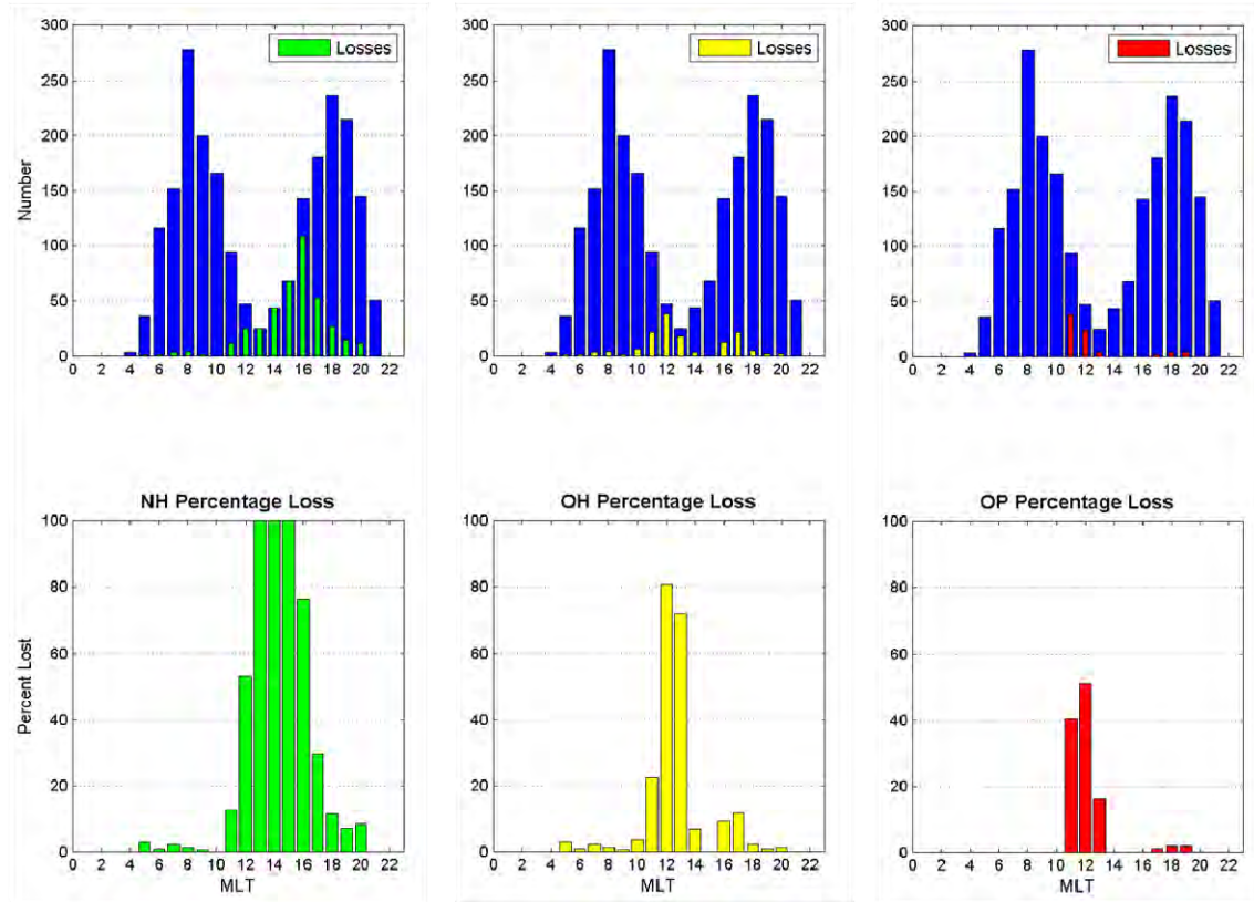
Figure 29. Top row: Data losses using 0.4 erg/cm 2 /s threshold for NH model (left), OH model (center), and OP model (right). Bottom row: Percentage of available DMSP passes lost in each MLT sector.
