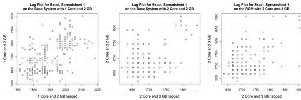
(a) Base System: (b) Base System: (c) RGM: 1 Core, 2 GB 2 Cores, 2 GB 2 Cores, 2 GB
