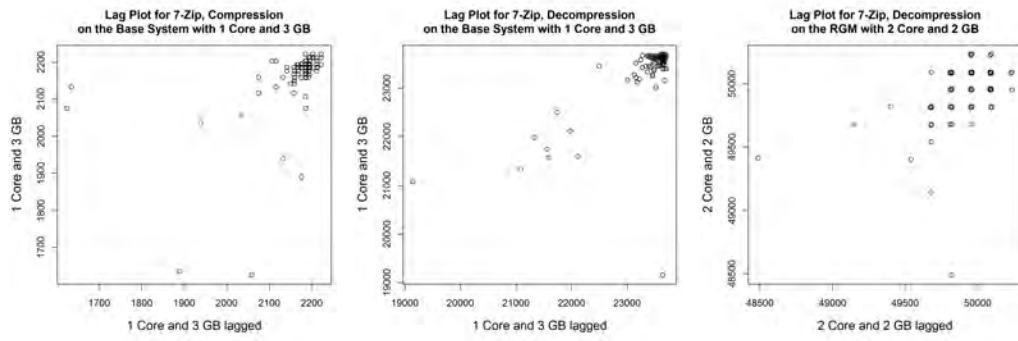
(a) Base System - Compression: (b) Base System - Decompression: (c) RGM - Decompression: 1 Core, 3 GB 1 Core, 3 GB 2 Cores, 2 GB
