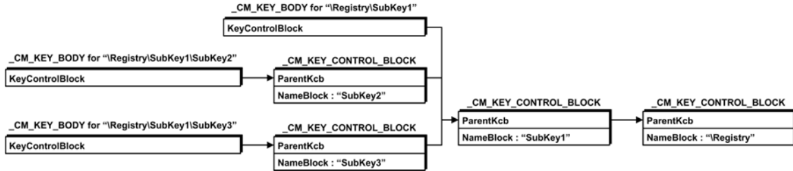
Figure 2.7: Example of the Relationship of the Key Object Related Structures
