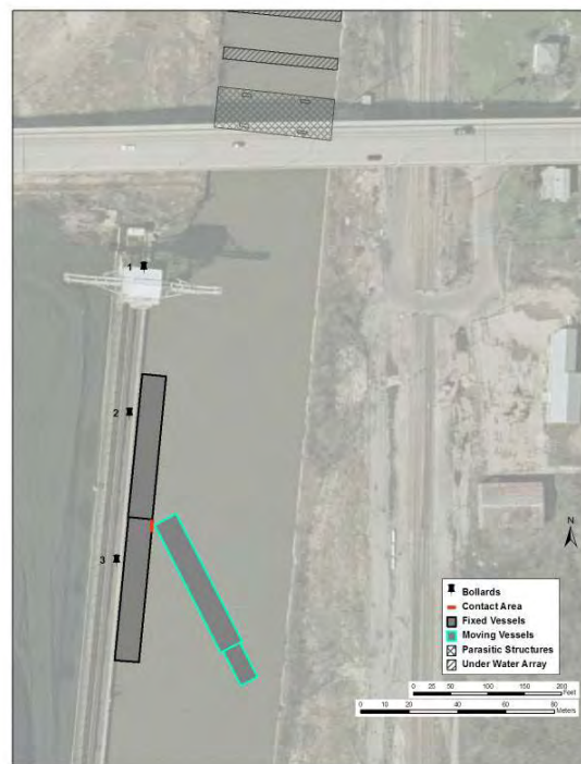
Figure 7. Sparking potential testing scenario for a tow with barges in parallel, 5 February 2011.
