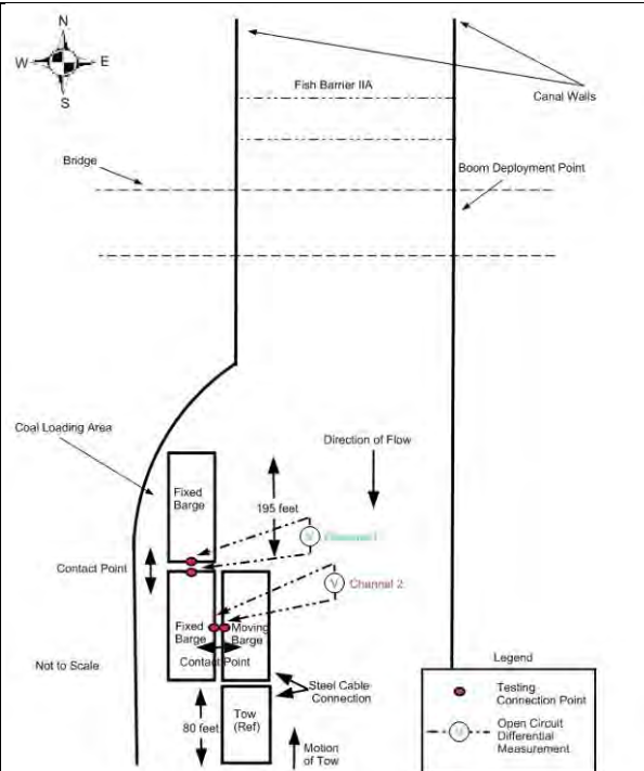
Figure 8. Instrumentation for testing of assembling a tow with barges in parallel.
