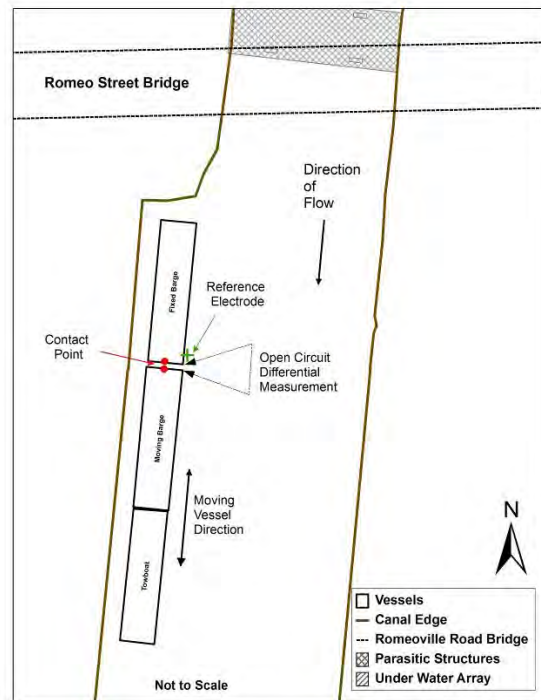
Figure 6. Instrumentation for testing of a tow with barges in series.
