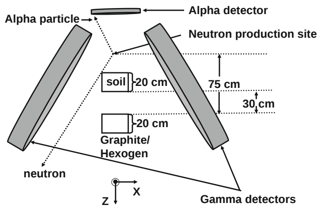
Fig. 2 Top view of the simulation environment showing the placement of objects along the neutron beam axis
