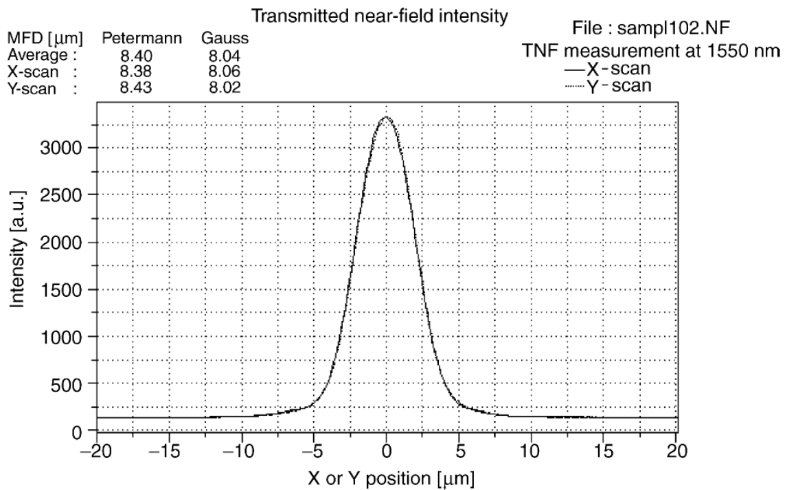
Figure 6: Intensity as a Function of Distance From Core's Center [6]
