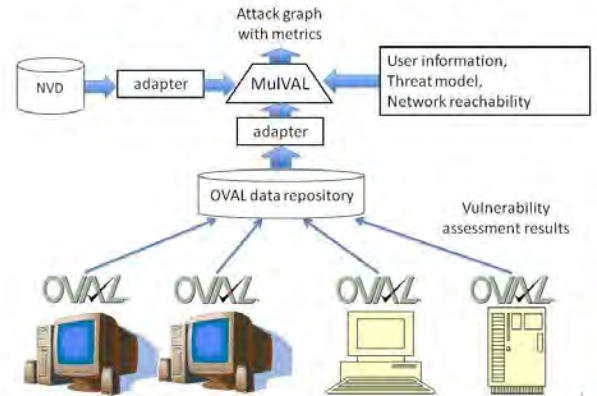
Figure 2. MulVAL attack-graph tool-chain
