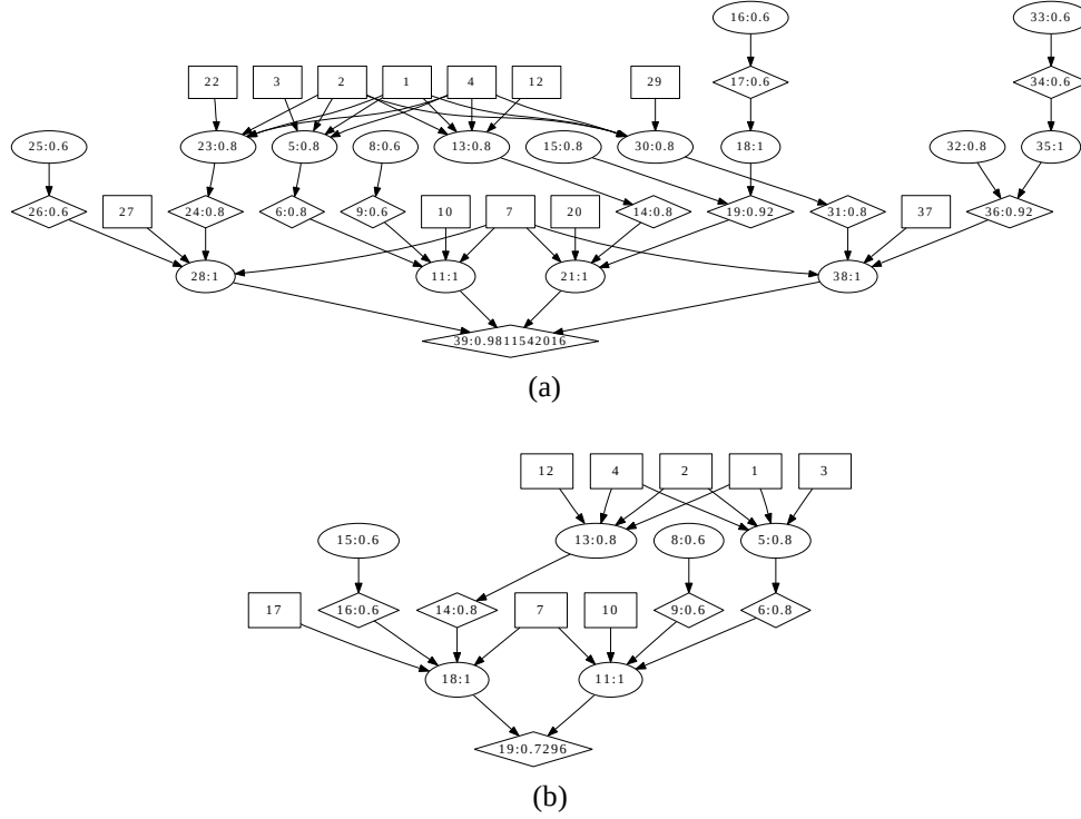
Figure 5. Attack graphs with modeling artifacts for capturing hidden correlations
