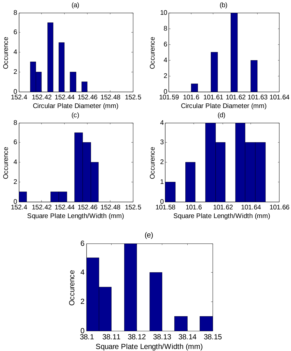
Figure 12: Histograms for the dimensions of (a) 6" Circular Plate, (b) 4" Circular Plate, (c) 6" Length/Width Square Plate, (d) 4" Length/Width Square Plate, and (e) 1.5" Length/Width Square Plate
