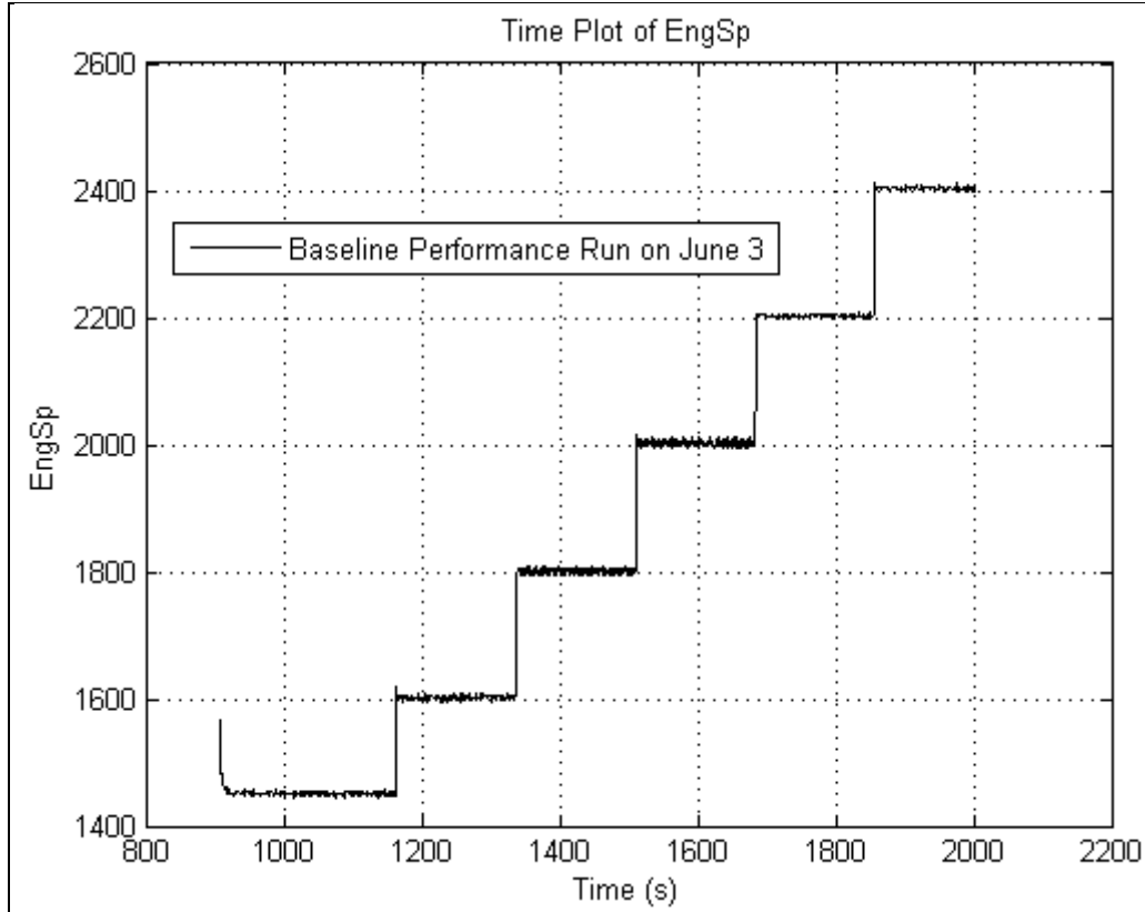
Figure 2. Typical stepped control of engine speed for a performance run.
