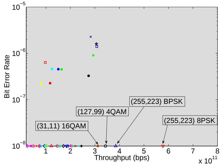
Figure 4.18: Throughput vs. \text{BER} < 10^{-5} for all modulations, 44 transmitters and 352 receivers for two-ray model.
