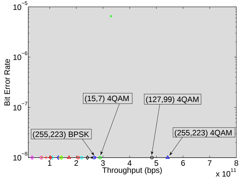
Figure 4.17: Throughput vs. \text{BER} < 10^{-5} for all modulations, 62 transmitters and 248 receivers for two-ray model.
