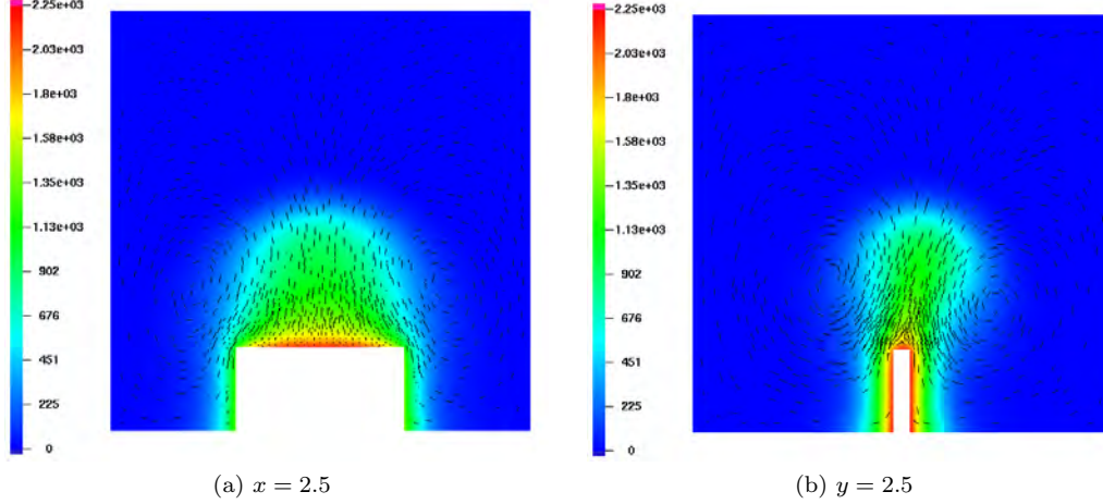
Figure 4: x (4a) and y (4b) interior cutplane views of the truth solution for (\text{Gr}, \phi) = (6000, 0.2) . Color contours show the temperature field and the overlaid velocity vectors indicate the circulatory nature of the flow.
