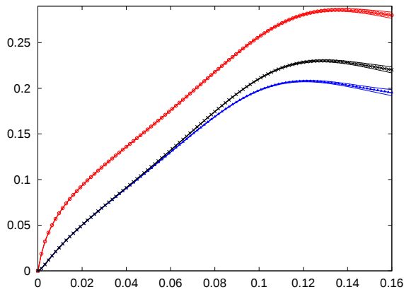
(e) (Gr, \phi) = (6000, 0.2)
