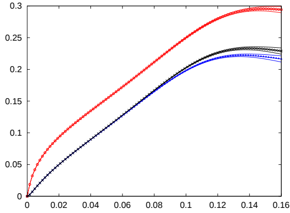
(c) (Gr, \phi) = (5000, 0.1)
