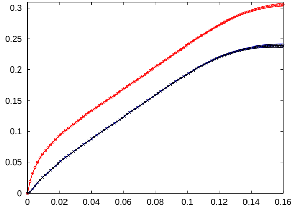
(a) (Gr, \phi) = (4000, 0)
