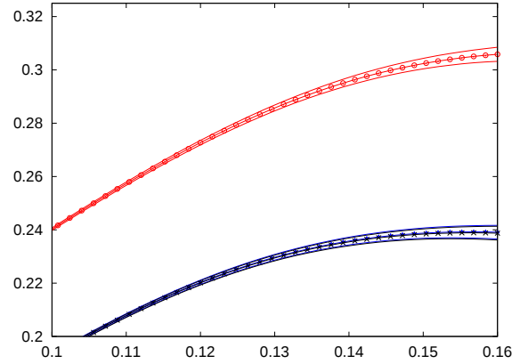
(b) (4000, 0) , Zoom near t_f
