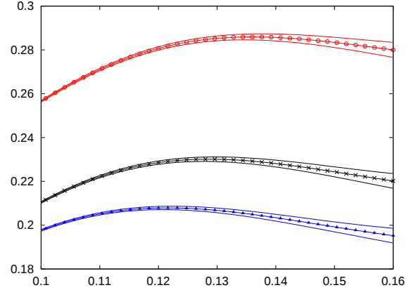
(f) (6000, 0.2) , Zoom near t_f
