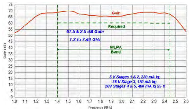
Figure 5. WLPA Small-Signal Gain vs. Frequency
