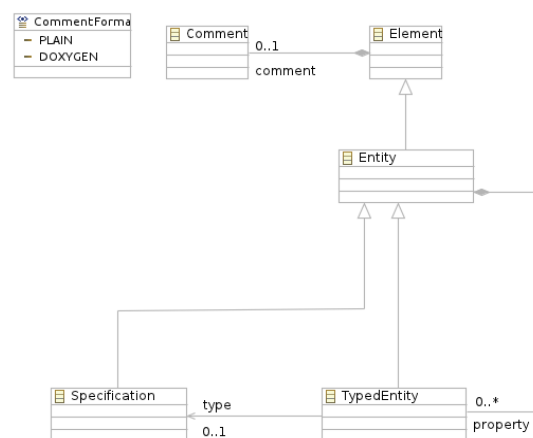
Drawing 1: Metamodel - Core
