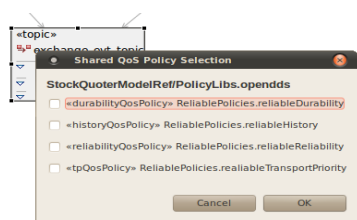
Drawing 24: DCPS Model Editor - shared policy values
