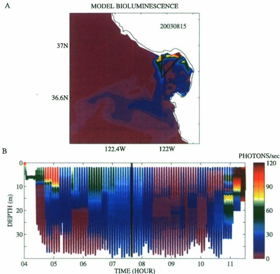
Figure 9. (a) Surface and (b) subsurface (along the REMUS transect) model-predicted BL distributions. Solid vertical line indicates location of the M1 mooring.
