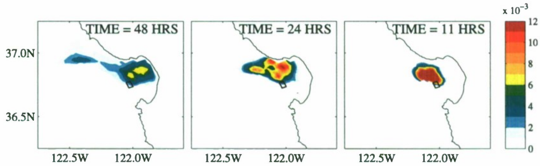
Figure 8. Adjoint passive tracer distributions on 15 August.
