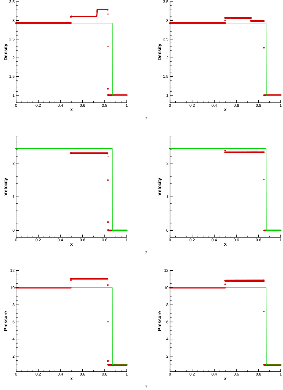
Figure 8.3: Density, velocity and pressure for Example 3. t = 0.1 . N_x = 1000 . Solid line: the exact solution. Symbol: the numerical solution. Left: exact Riemann solution without subcell resolution; Right: subcell resolution and with the line path instead of the exact Riemann solution.
