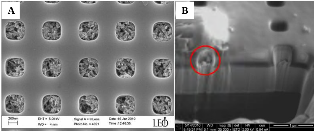
Figure 3: Nanoscale vias filled with TiO 2 nanoparticles imaged A) top down before Pt capping and B) cross section of filled via after Pt capping.
