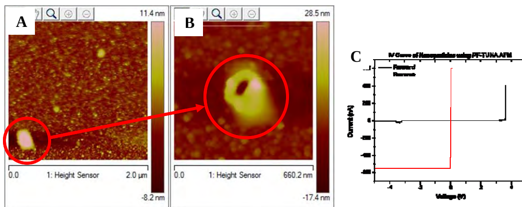
Figure 2: Tapping mode AFM scans A) before electrical biasing and B) after electrical biasing. C) Shows corresponding forward ( -5\text{V} \rightarrow 5\text{V} ) and reverse ( 5\text{V} \rightarrow -5\text{V} ) IV sweeps of biasing the nanoparticles.
