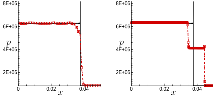
Figure 11: Computed pressure for the Heaviside Example 4.2 at t = 3 \times 10^{-7} . Solid line: reference solution. Dashed line with symbols: numerical solution. Left: WENO5/SR with N = 50 , CFL=0.1, N_r = 10 ; right: splitting WENO5 with N = 300 , CFL=0.01.
