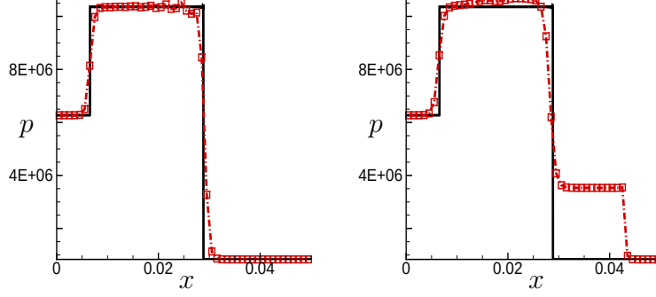
Figure 15: Computed pressure for the Heaviside Example 4.3 at t = 2 \times 10^{-7} . Solid line: reference solution. Dashed line with symbols: numerical solution. Left: WENO5/SR with N = 50 , \text{CFL}=0.1 , N_r = 10 ; right: splitting WENO5 with N = 50 , \text{CFL}=0.01 .
