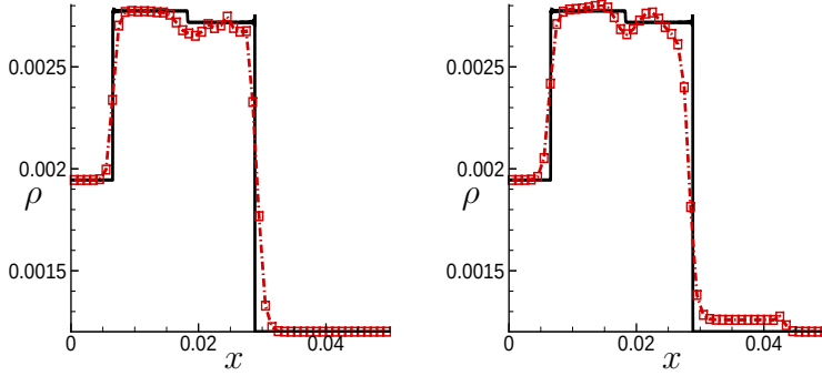
Figure 17: Computed density for the Heaviside Example 4.3 at t = 2 \times 10^{-7} . Solid line: reference solution. Dashed line with symbols: numerical solution. Left: WENO5/SR with N = 50 , CFL=0.1, N_r = 10 ; right: splitting WENO5 WENO5 with N = 50 , CFL=0.01.
