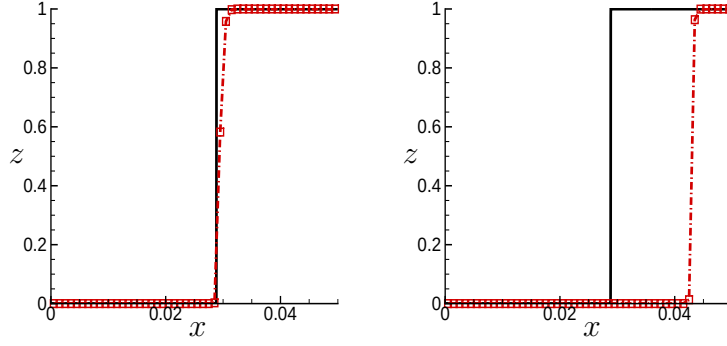
Figure 18: Computed mass fraction for the Heaviside Example 4.3 at t = 2 \times 10^{-7} . Solid line: reference solution. Dashed line with symbols: numerical solution. Left: WENO5/SR with N = 50 , CFL=0.1, N_r = 10 ; right: splitting WENO5 WENO5 with N = 50 , CFL=0.01.
