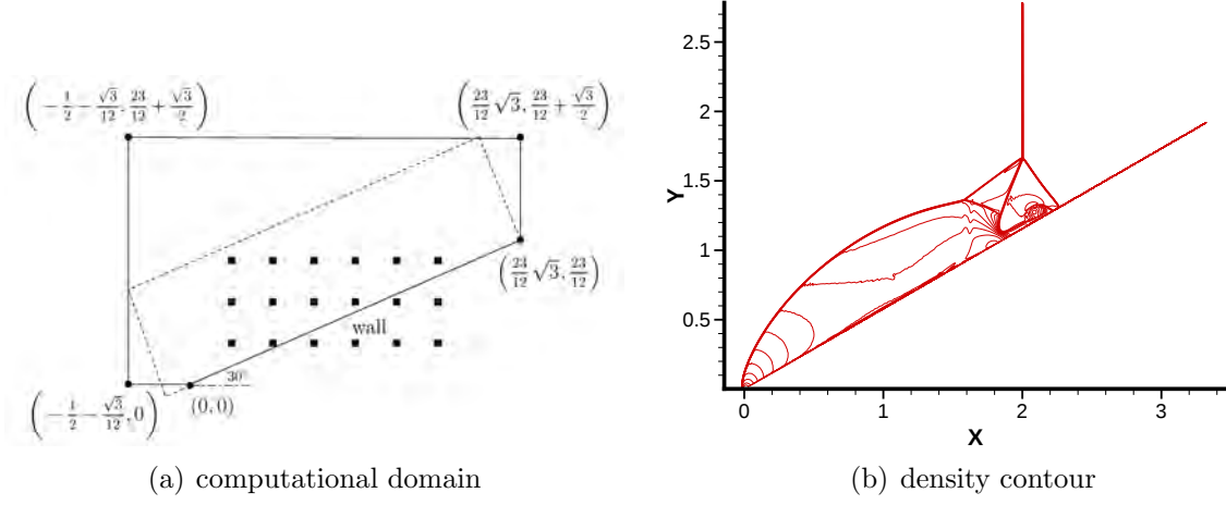
Figure 3.2: Left: The computational domain (solid line) of the double Mach reflection problem. The dashed line indicates the computational domain used in [7, 15]. The square points indicate some of the grid points near the wall. Illustrative graph, not to scale. Right: Density contour of double Mach reflection, 30 contour lines from 1.731 to 20.92. h = 1/320 .
