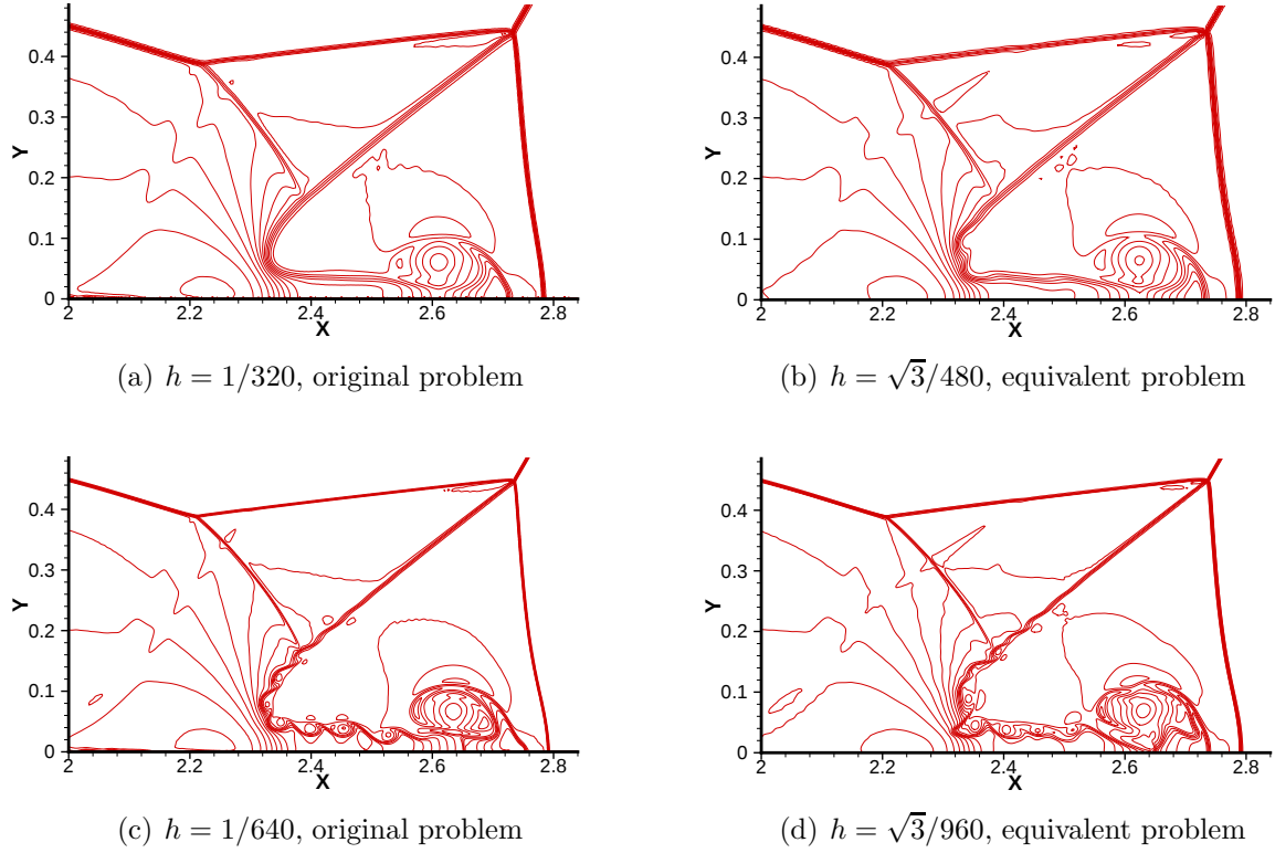
Figure 3.3: Density contours of double Mach reflection, 30 contour lines from 1.731 to 20.92. Zoomed-in near the double Mach stem. The plots in the left column are rotated and translated for comparison.
