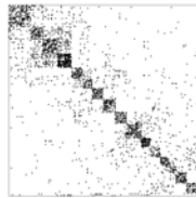
(n) School 80, K = 4
