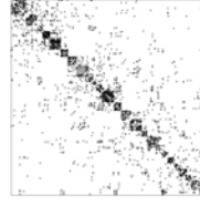
(c) School 21, K = 6
