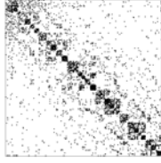
(j) School 66, K = 6
