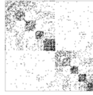
(g) School 38, K = 5
