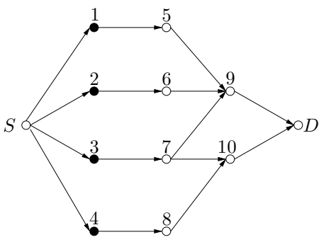
Fig. 3. A network with capacity strictly less than the cut-set bound.
