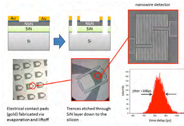
Figure 7: Nanowire fabrication.
