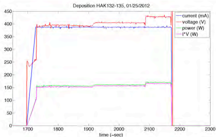
Figure 5. Current, voltage, and power readings from the power supply during a DC magnetron sputtering event. Voltage jumps correspond with Ar pre-sputtering, Ar+N 2 pre-sputtering, and the opening of the shutter.
