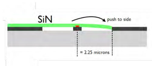
Figure 12: Mechanical alignment.
