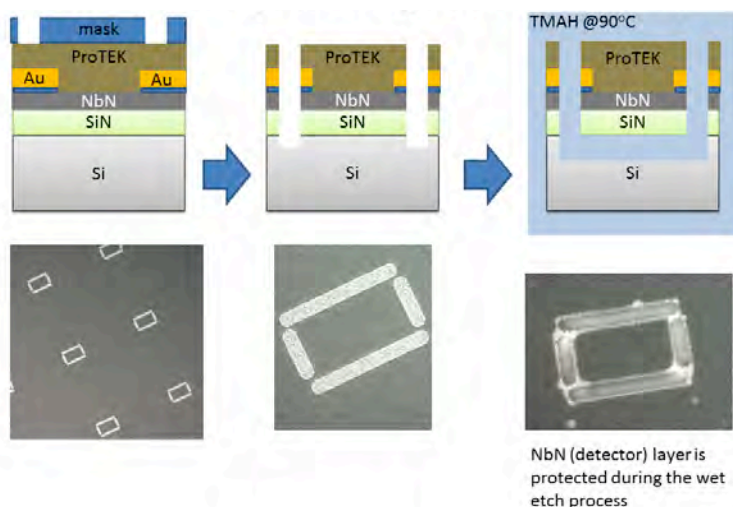
Figure 8: Current membrane under-cut process.
