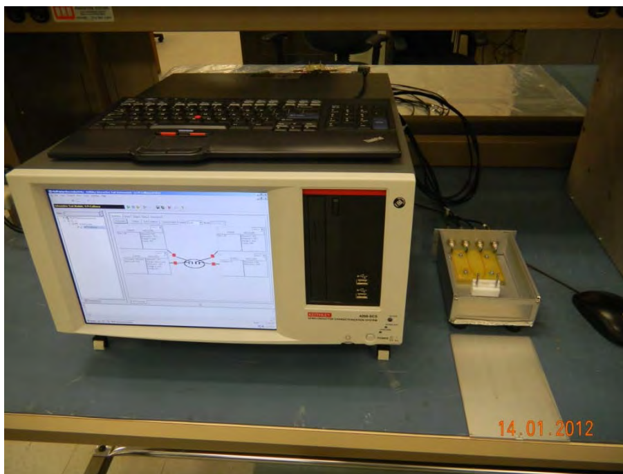
Figure 17. Bulk resistivity measurement setup. Keithley 4200 SCS on the left and sample holder on the right.
