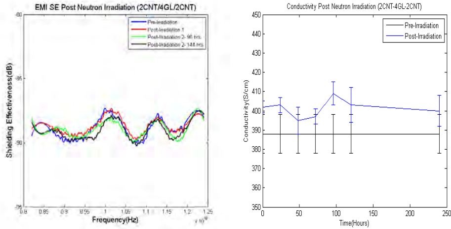
Figure 37. Changes over time to EMI-SE (left) and conductivity (right) of 2CNT/4GL/2CNT sample after neutron irradiation.
