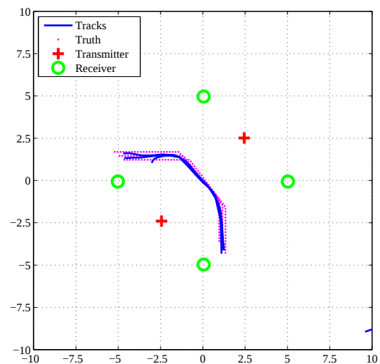
Figure 4. Scenario 2 ML-PDA estimated tracks
