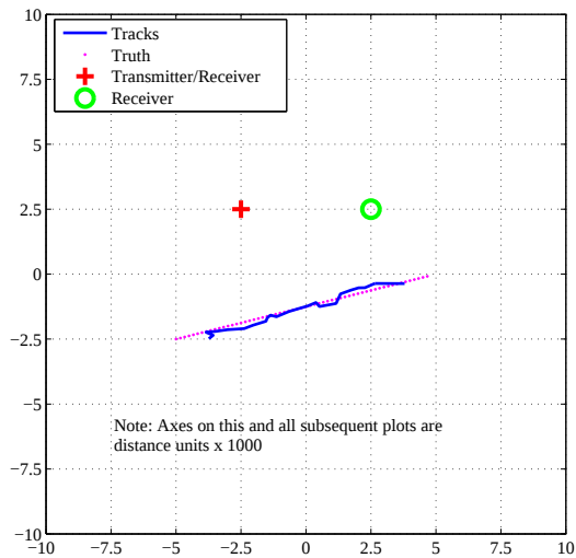
Figure 1. Scenario 1 ML-PMHT estimated tracks
