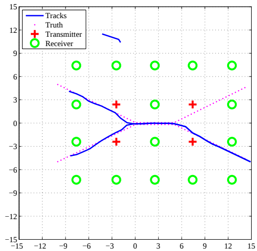
Figure 9. Scenario 5 ML-PMHT estimated tracks
