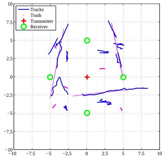
Figure 7. Scenario 4 ML-PMHT estimated tracks
