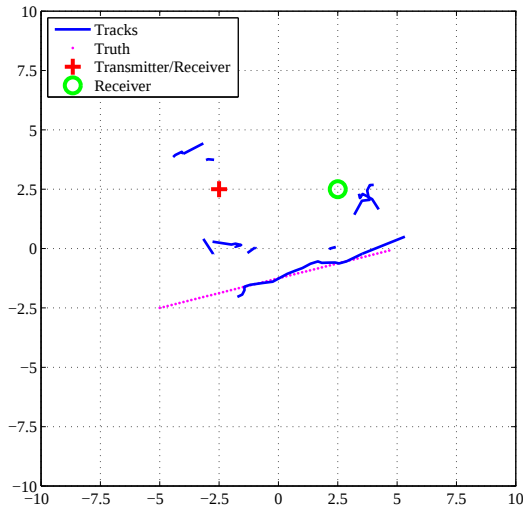
Figure 11. Scenario 1 ML-PMHT estimated tracks with Rayleigh clutter
