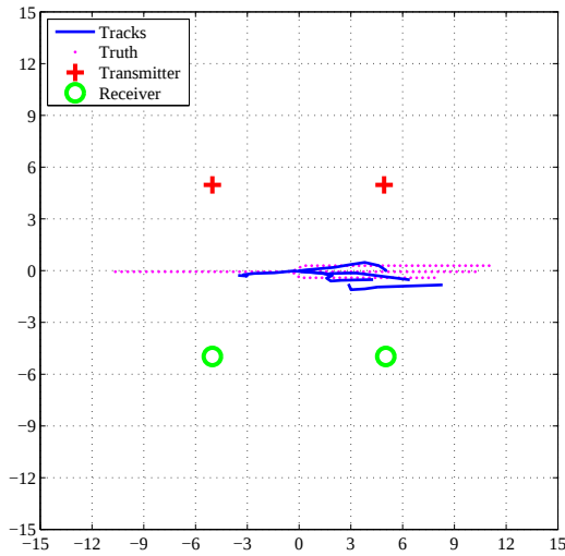
Figure 5. Scenario 3 ML-PMHT estimated tracks
