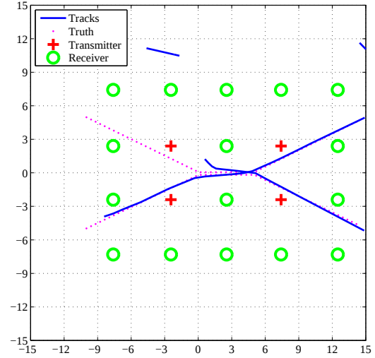
Figure 10. Scenario 5 ML-PDA estimated tracks
