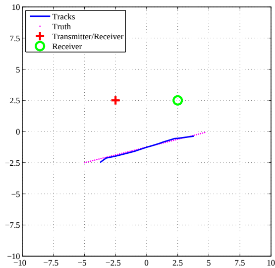
Figure 2. Scenario 1 ML-PDA estimated tracks
