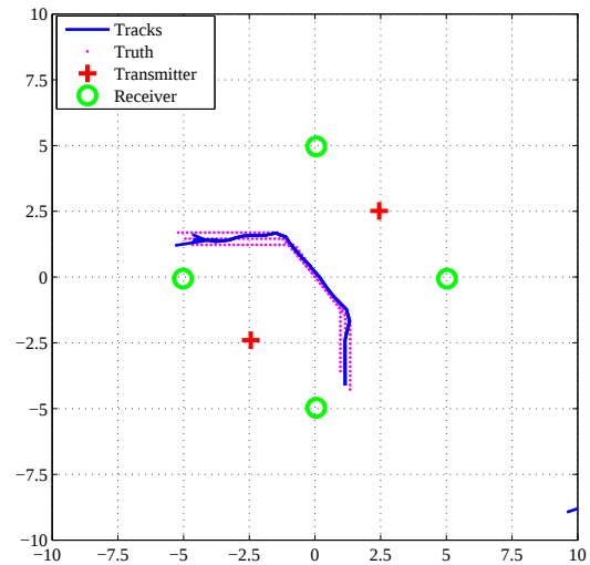
Figure 3. Scenario 2 ML-PMHT estimated tracks
