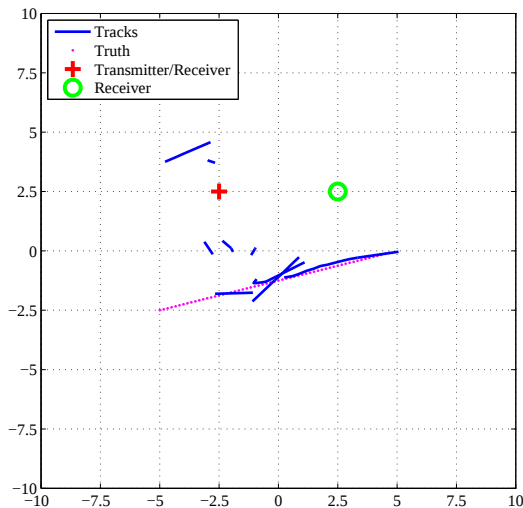
Figure 12. Scenario 1 ML-PDA estimated tracks with Rayleigh clutter
