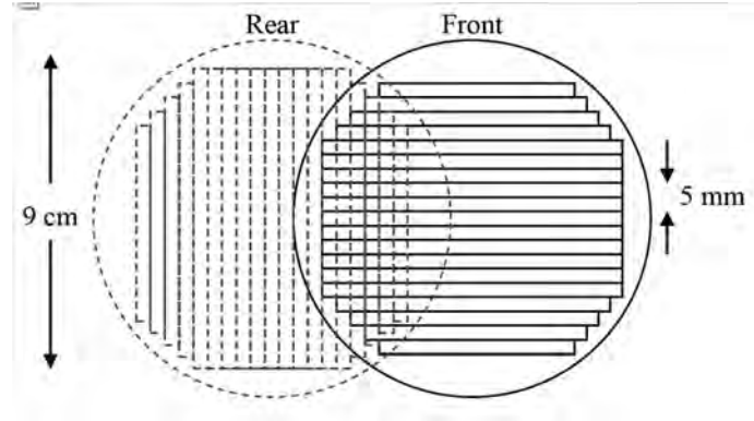
Figure 26. The configuration of the PHDs detector crystal [75].
