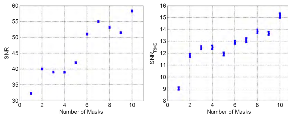
Figure 46. Left: SNR versus number of masks used, Cd-109 with background, 1 hr detection time. Right: \text{SNR}_{\text{RMS}} versus number of masks used, Cd-109 with background, 1 hr detection time.
