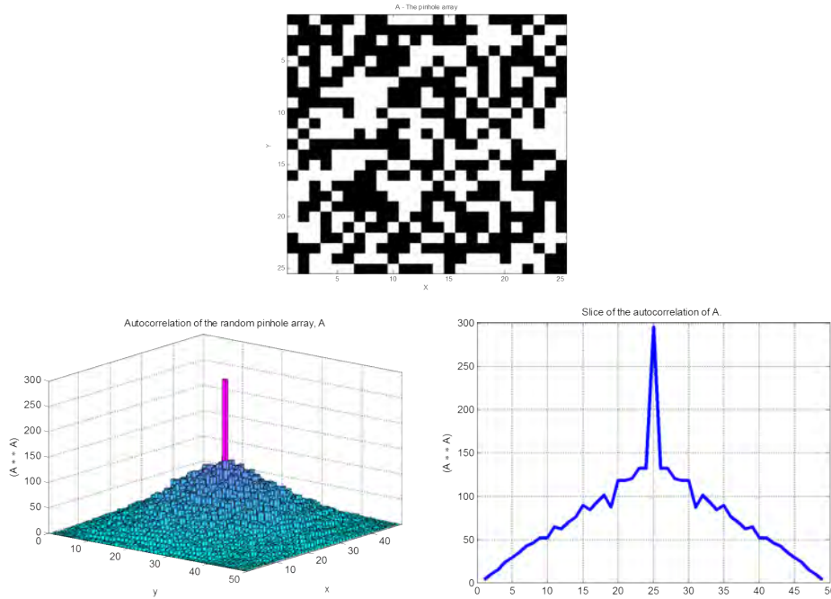
Figure 3. Top: A random pinhole array, A . Bottom-Left: The autocorrelation of the pinhole array, A . Bottom-Right: A slice in one dimension of the autocorrelation of A .
