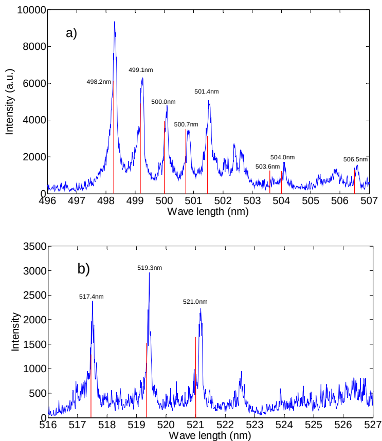
Figure 2. Emission spectra acquired from a laser excitation of 532nm (35mJ/p). Ti atomic spectra from NIST database is marked by red lines.
