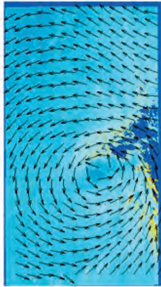
Figure 5: Malakas 22 Sep 2010, 20:30 UTC. Effect of using SLP-filtered wind directions to improve CMOD5N retrievals in high wind and low incidence angle conditions. (a) raw speeds using GD/NURC directions. (b) Retrieved speeds using SLP-filtered wind directions (1 iteration). (c) Retrieved speeds using SLP-filtered wind directions (2 iterations). The region of no solution is the dark blue. Note how it shrinks when SLP-filtered directions are used.
