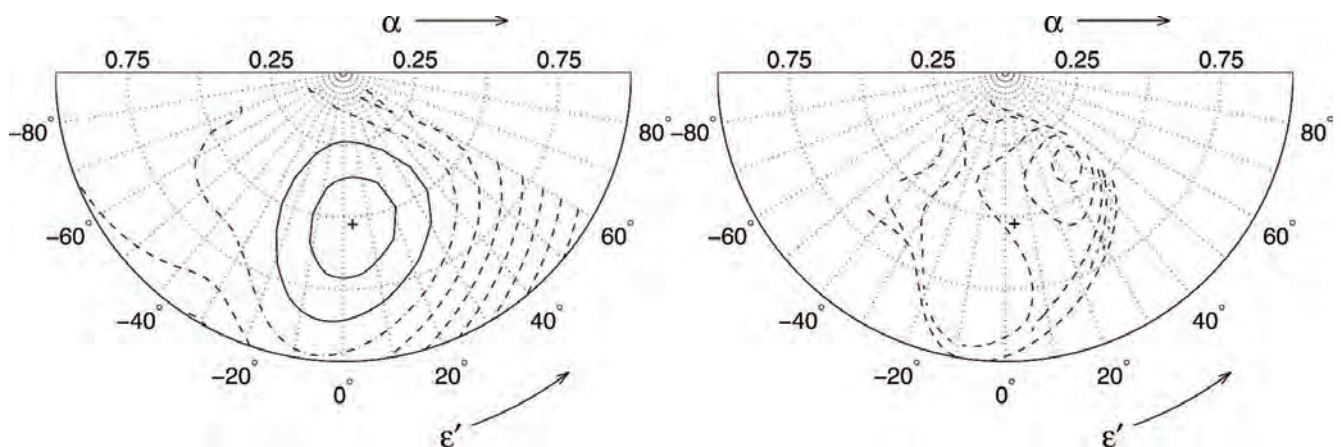
Figure 13: (a) Figure 4 and (b) Figure 7 from Foster (2005). The original captions are: FIG. 4. Linear instability growth rate a_0 as a function of angle from azimuthal wind \epsilon' = \epsilon - 90^\circ and wavenumber \alpha for r = 40\text{km} and \Delta T = -5\text{ K} . Solid lines denote positive growth rates, dash-dotted lines denote zero growth, and dashed lines denote negative growth rates. Contour interval is 0.005 (nondimensional). The equivalent plot for neutral stratification is very similar with overall reduced growth rates and the peak shifted toward larger \epsilon' . FIG. 7. First Landau coefficient a_1 corresponding to the conditions in Fig. 4 for a_0 > 0 . The a_0 = 0 contour is shown as dash-dot. Contour interval is 0.0005 (nondimensional).
