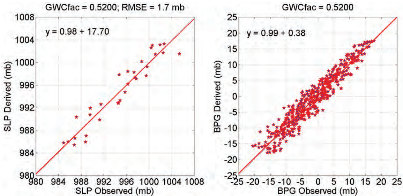
Figure 4: Malakas 22 Sep 2010, 20:30 UTC. (a) Comparison of sonde splash pressure with SAR-derived pressure. (b) Comparison of bulk surface pressure differences between all pairs of drop sondes and the SAR SLP.
