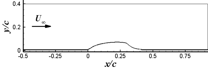
Figure 3. Geometry of wall-mounted hump
