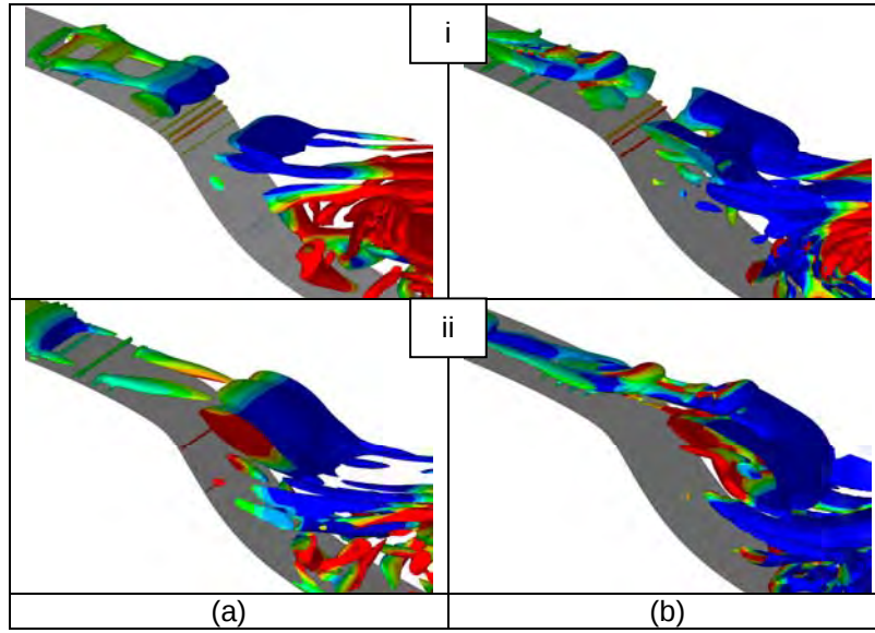
Figure 13. Instantaneous iso-surface of the swirl strength colored by the cross-stream velocity for the (a) spanwise oriented and (b) streamwise oriented slots at: (i) \phi = 180^\circ (end of expulsion phase), (ii) \phi = 270^\circ (end of ingestion phase)
