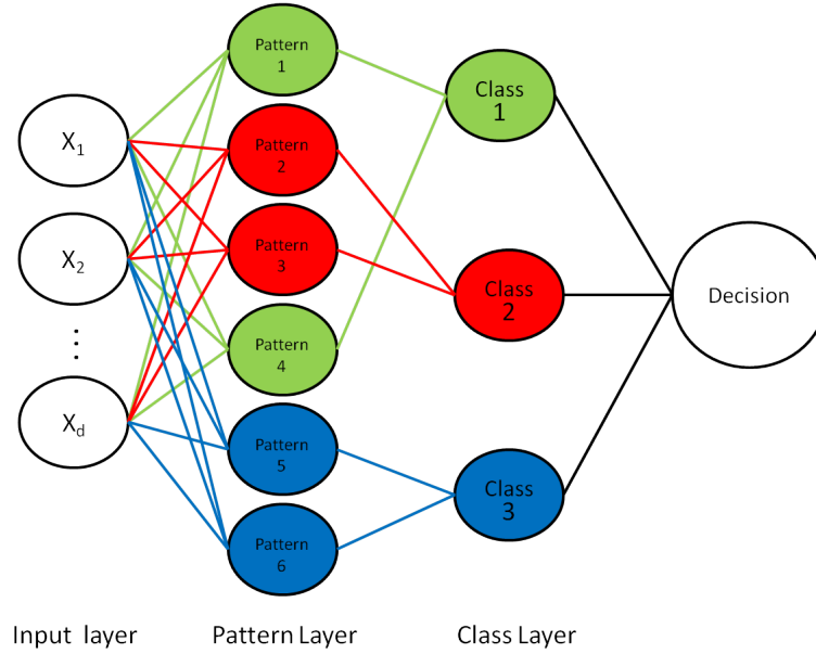
Figure 12. Example of a PNN
