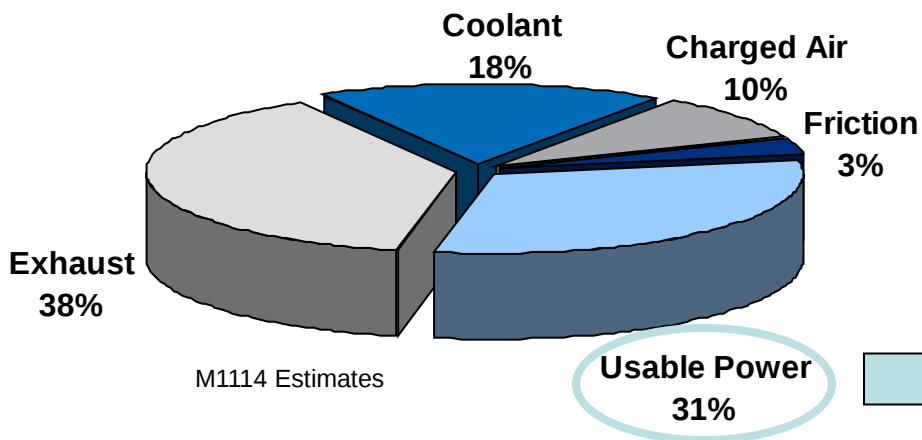
Engine Energy Balance
