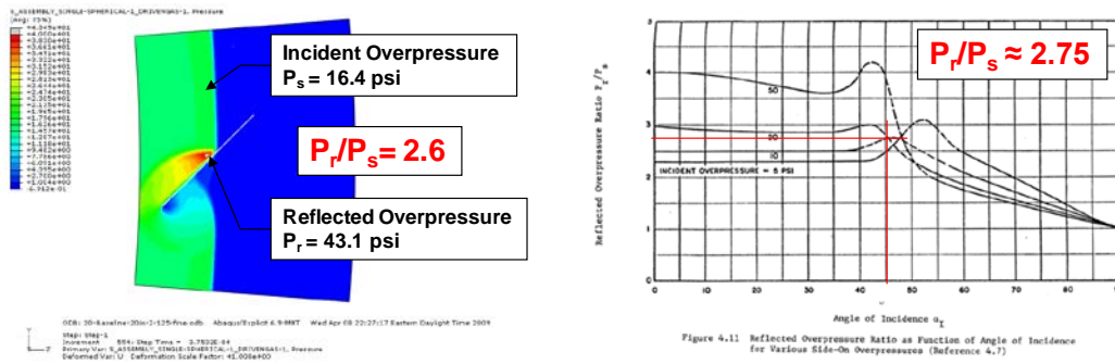
Figure 9. Comparison of results between oblique reflection model in Abaqus/CEL model and empirical data.
