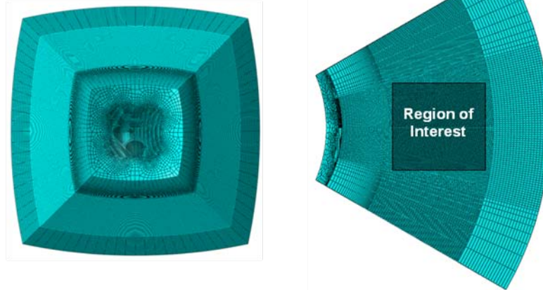
Figure 12. Mesh used for Eulerian air domain – 2.6 million elements total.
