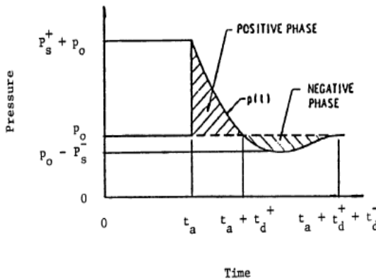
Figure 1. Ideal blast wave (DOE/TIC-11268, 1981).
