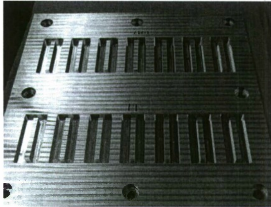
Fig. 16. Aluminum rib in channel plate before being filled with support materials.
