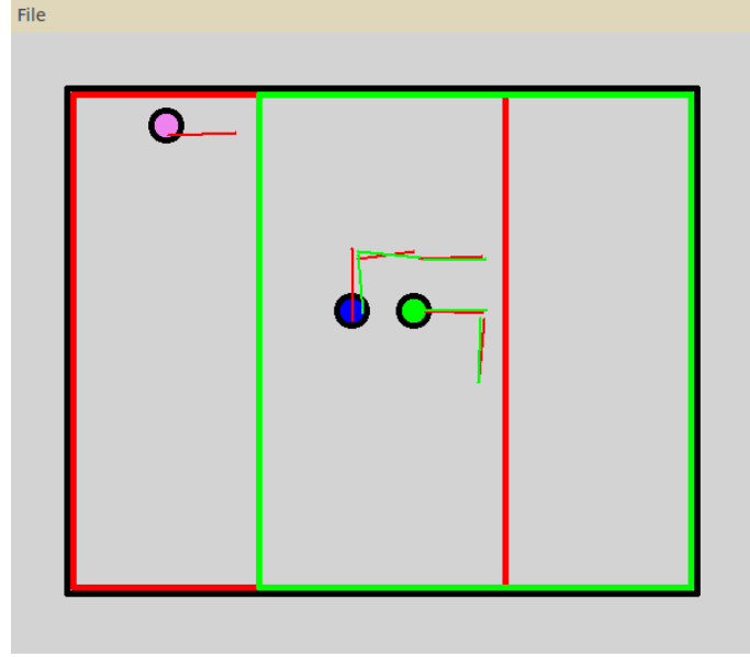
Figure 2: Simulator example. This 2D world contains 3 agents (pink, green and blue) and 2 overlapping cameras (red and green rectangles). Active tracks are shown as lines coloured as their corresponding camera. For example, green and blue agents are currently being tracked in both cameras, while the pink agent is only tracked in a single camera.
