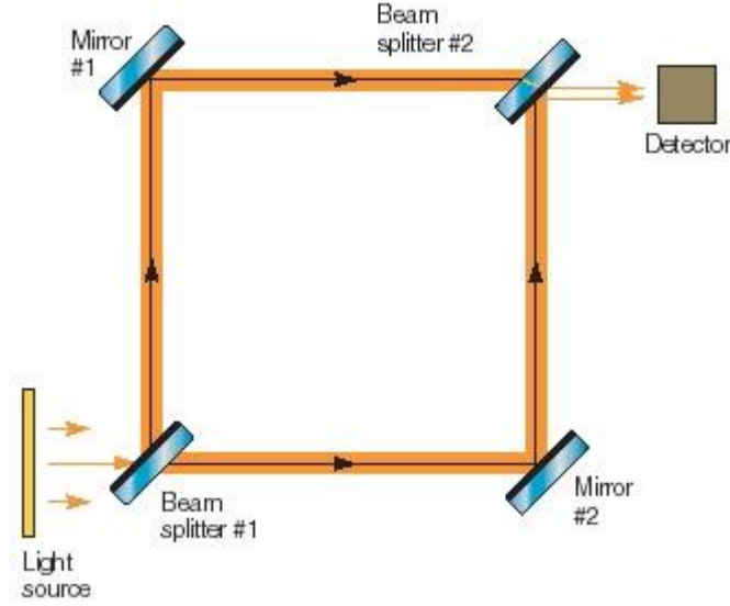
Figure 1.1: Mach-Zehnder Interferometer
