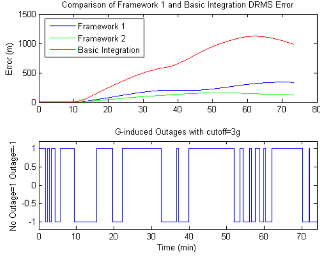
Figure 4.29: Dual INS G-Induced Outages with G Cutoff of 3G's
