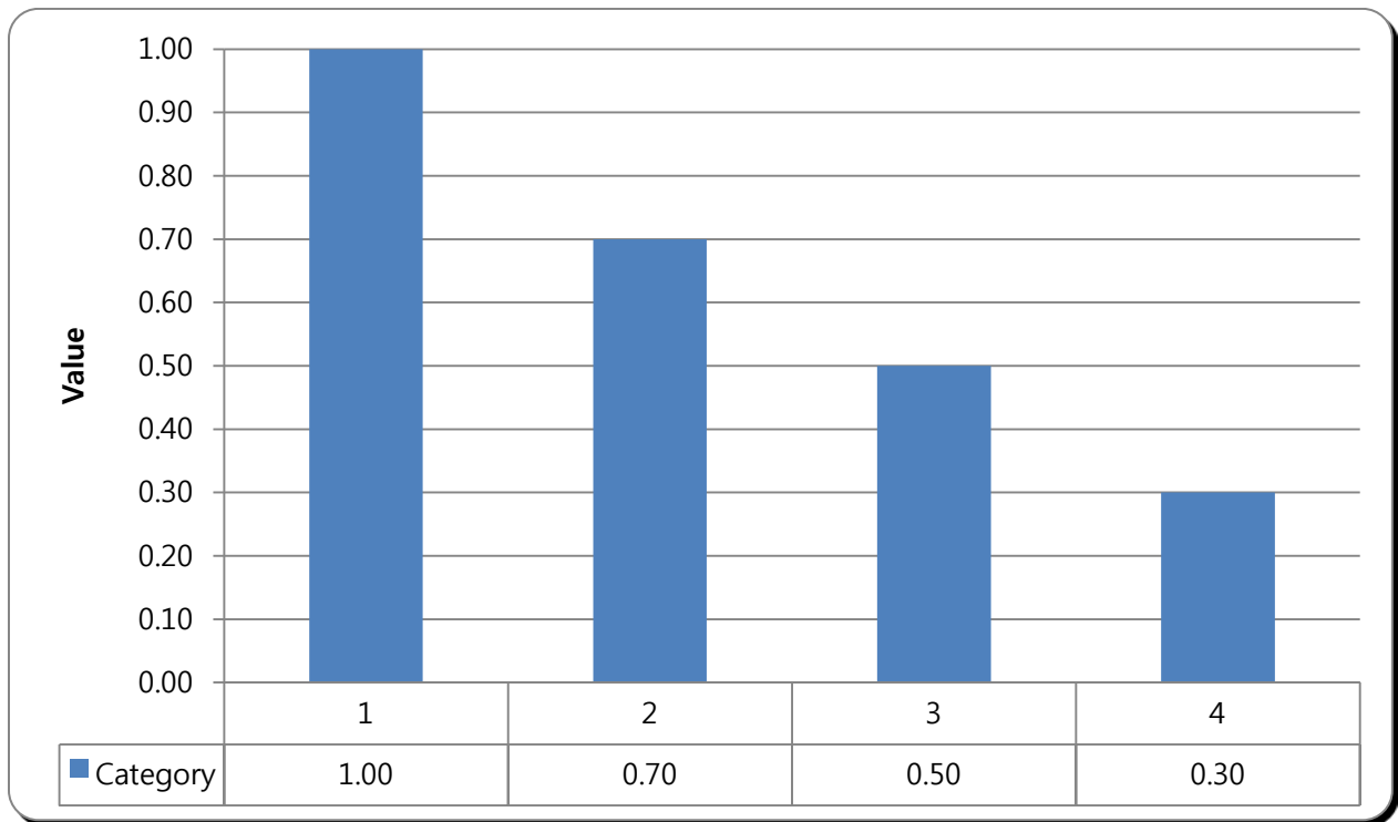
Figure 34 Commanders' Assessment
