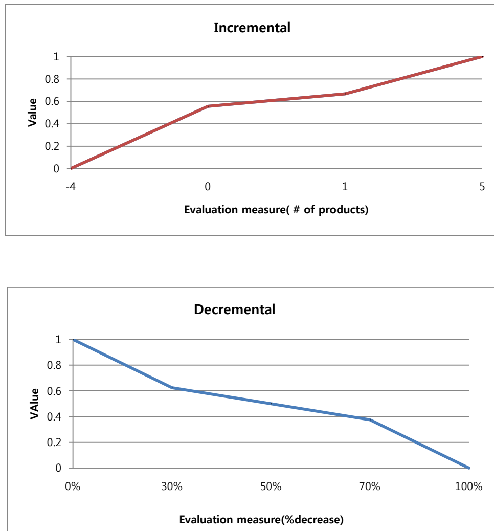
Figure 5 Piecewise SDVF
