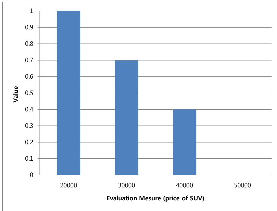
Figure 7 Categorical SDVF
