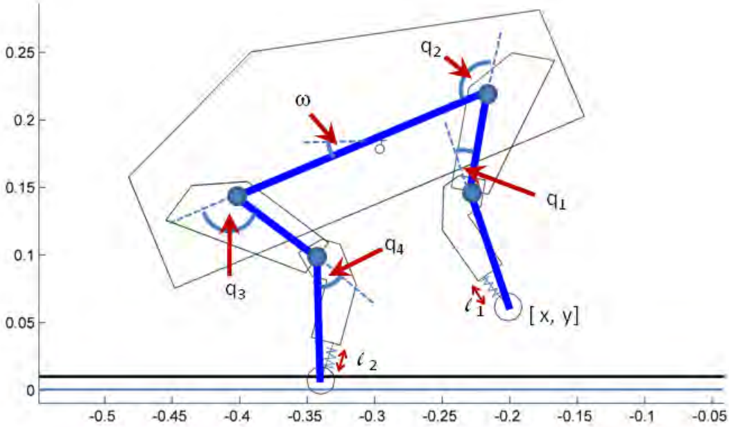
Figure 6-3: LittleDog model. The state space is \mathcal{X} = [\mathbf{q}, \dot{\mathbf{q}}, \mathbf{l}] , where \mathbf{q} = [x, y, \omega, q_1, q_2, q_3, q_4] , and \mathbf{l} = [l_1, l_2] are feet spring lengths used in the ground contact model. The diagram also illustrates the geometric shape of the limbs and body, information used for collision detection during planning.
