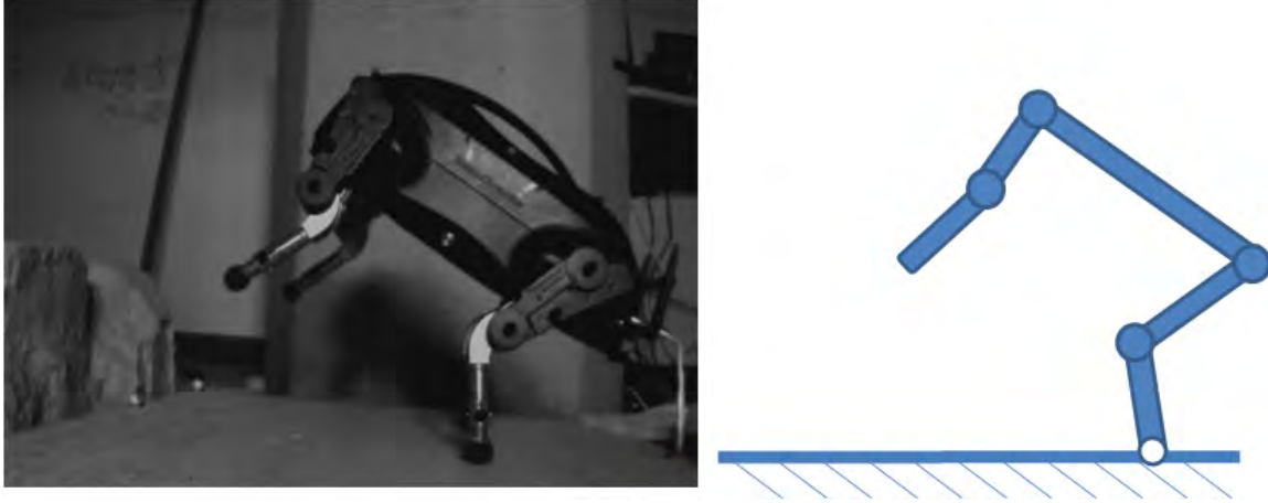
Figure 6-1: LittleDog robot, and a corresponding 5-link planar model (blue circles represent actuated joints, white circles represent passive joints)
