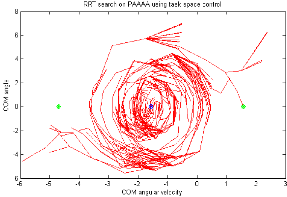
Figure 4-6: This figure shows the projection of an RRT tree built on a PAAAA system, showing the system COM angle and angular velocity. The projection of the root of the tree is shown by the blue circle, and the goal points are shown in green (wrapped around 2\pi ). One can see that this projection looks much like an RRT for a pendulum. Using the COM as a task space, the Task Space Guided RRT is able to quickly find plans for swing up on this system.
