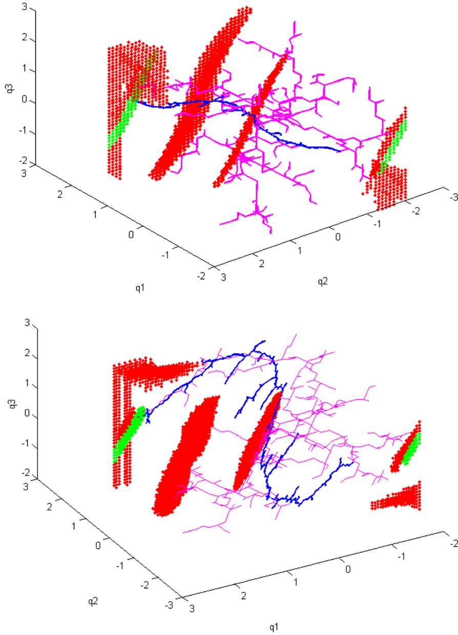
Figure 2-4: TOP/BOTTOM are two rotated views of the same 3D plot. This figure shows the configuration space view of an RRT tree (magenta), and a TS-RRT (blue), both for a 3-link arm. Obstacles (same as those shown in Figure 2-2) are shown by red dots, and the goal task point is shown by green dots in the configuration space. The standard RRT has good coverage in the space, as expected. Both trees converge to a collision free trajectory, but it clear that the TS-RRT is much more direct. ©2009 IEEE [Shkolnik and Tedrake, 2009].
