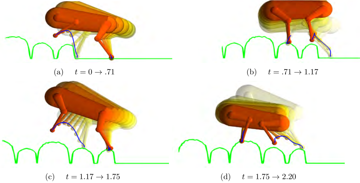
Figure 6-8: Bounding trajectory over logs
