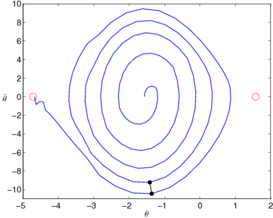
Figure 5-1: Example state space trajectory for the torque-limited, single link pendulum. Due to the torque limits at the shoulder, a swing up phase is necessary to drive the pendulum from the vertical downward position to the stationary upright position. The two black dots connected by a segment shows that the Euclidean metric is not a good measure of cost-to-go. ©2009 IEEE [Shkolnik et al., 2009].
