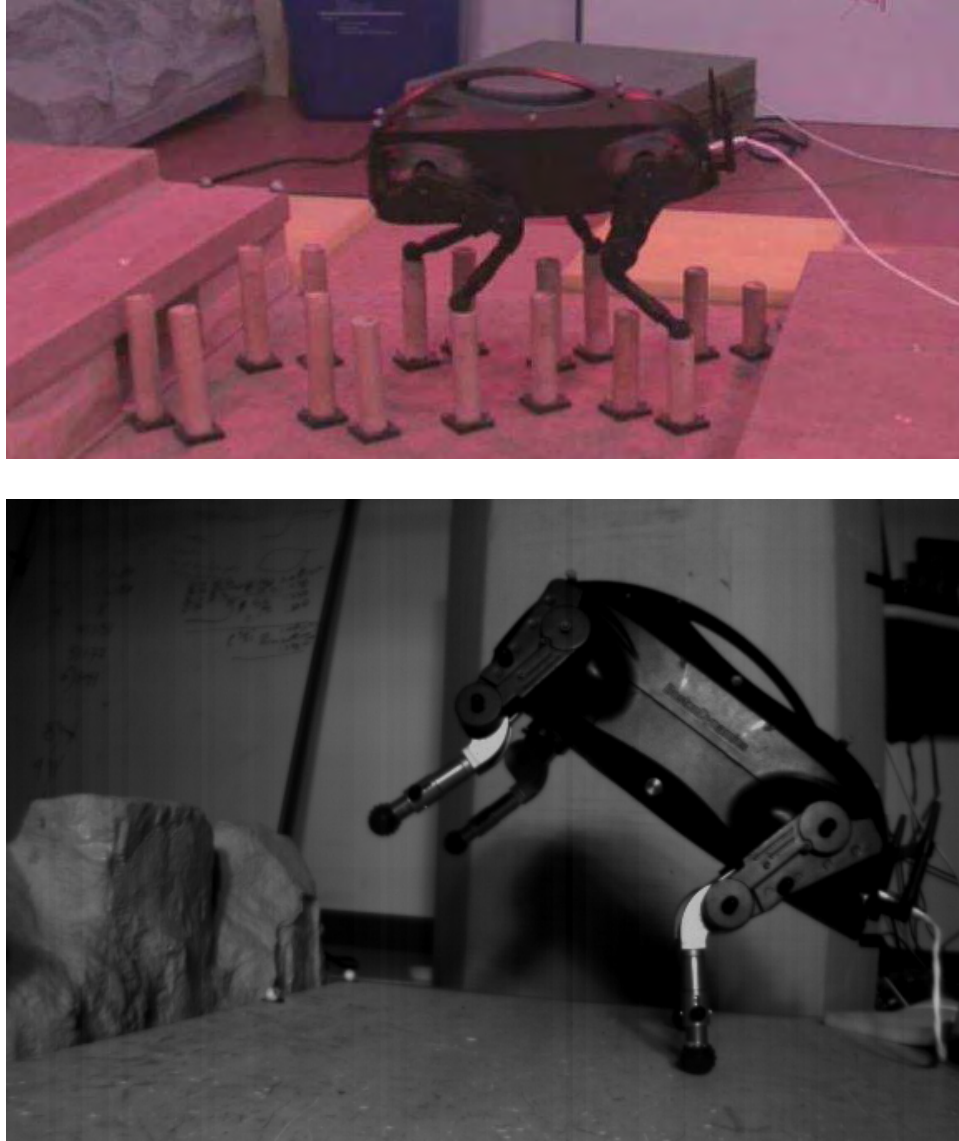
Figure 1-3: TOP: LittleDog robot walking on pegs. BOTTOM: LittleDog on hind legs.
