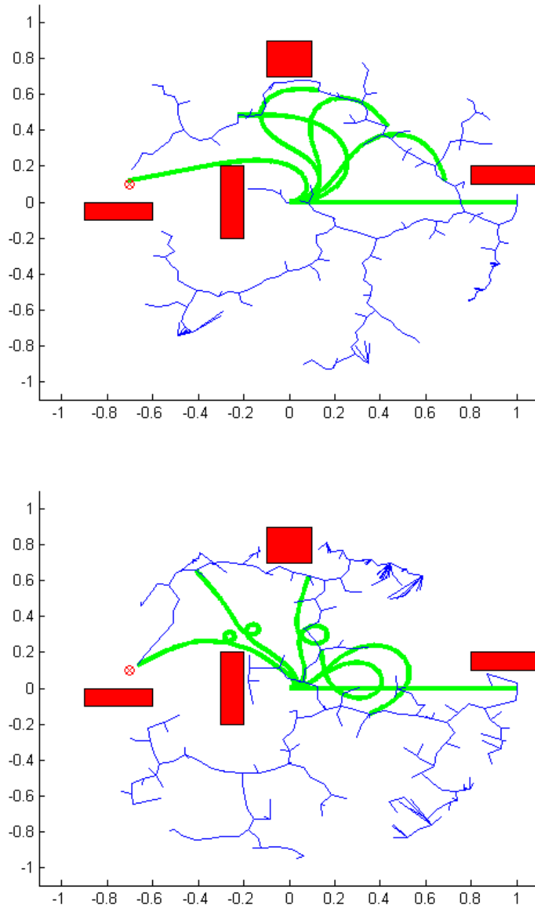
Figure 2-5: Two example trajectories and RRT plans, found with N = 1500 . Total computation time was less than one minute. ©2009 IEEE [Shkolnik and Tedrake, 2009].
