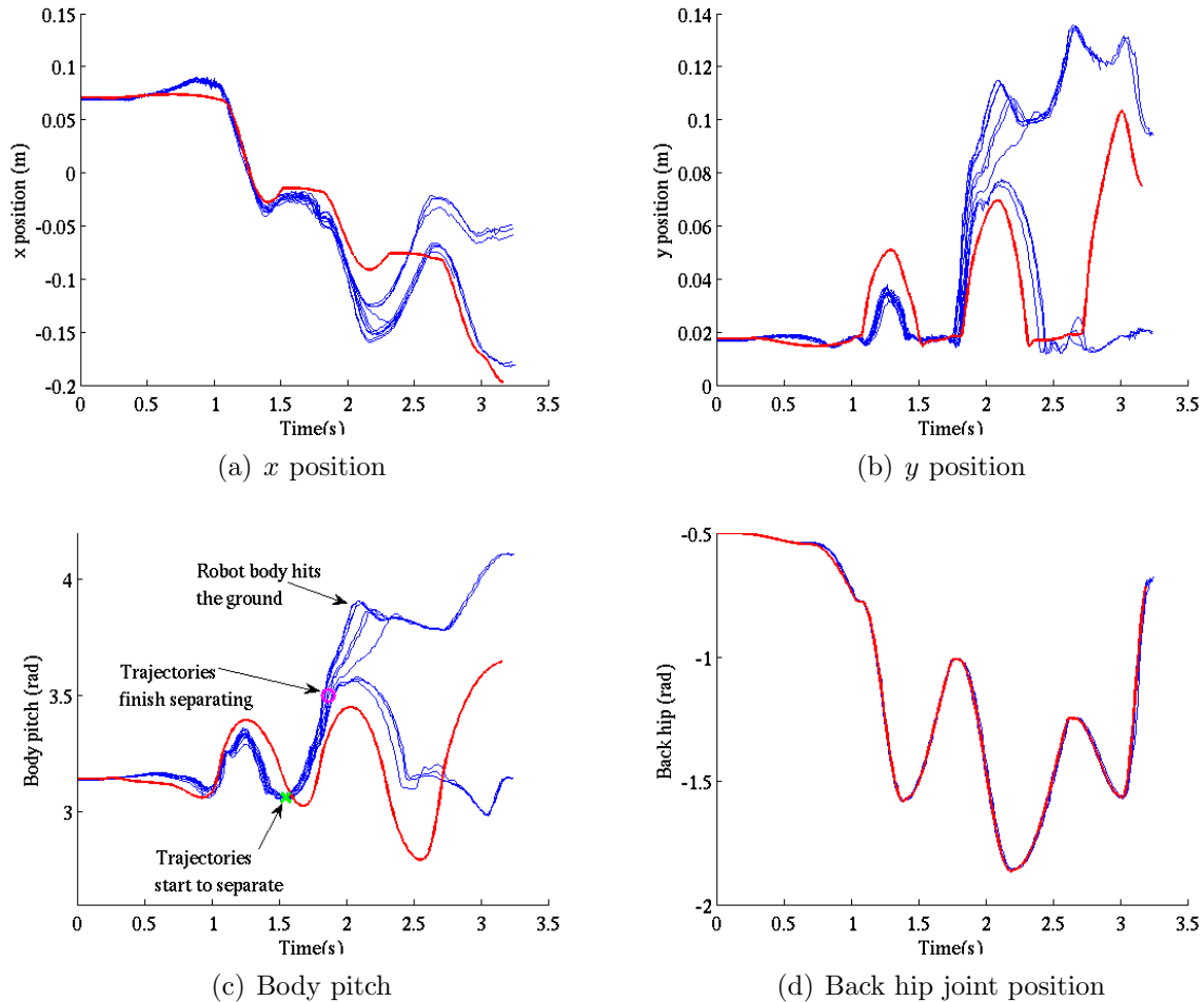
Figure 6-11: LittleDog Model compared to Actual Trajectories for a bounding motion on flat terrain: Unactuated coordinates: x (top left), y (top right), and body pitch (bottom left); trajectory of one of the joints (bottom right). The thick red line shows a trajectory generated by planning with RRT's using the simulation model. The blue lines are 10 open-loop runs of the same trajectory on a real LittleDog robot. It is clear that the model captures the actuated dynamics very well. The unactuated dynamics are highly nonlinear, but the model captures much of the system behavior. The response of the robot itself is unstable, even from very similar starting conditions. Figure by Michael Levashov.
