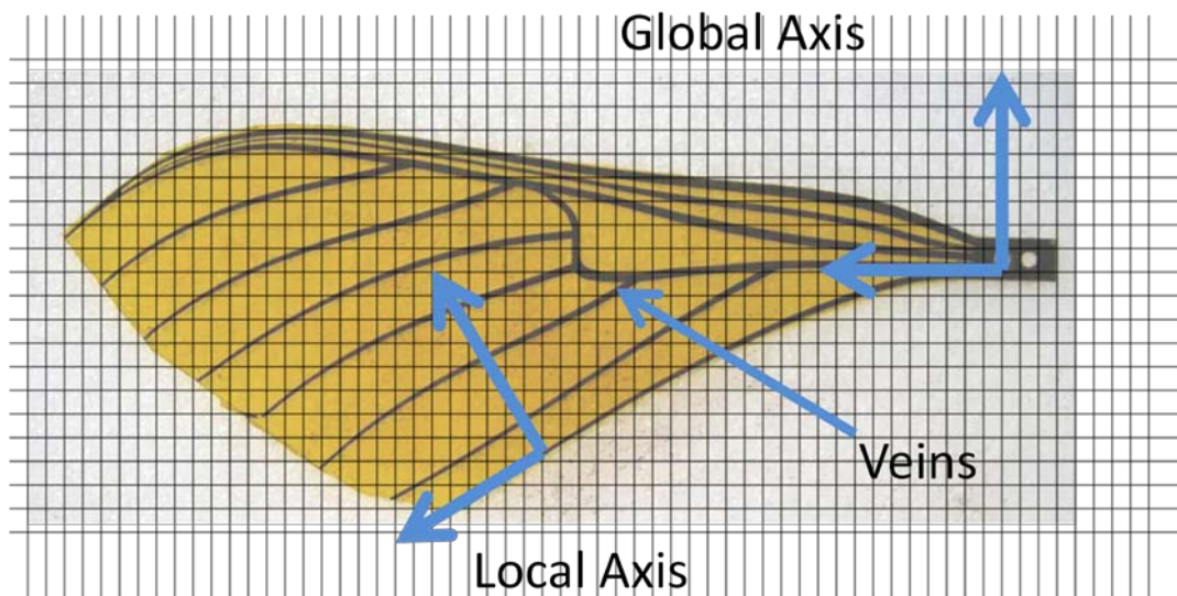
Figure 2.1: The Manufactured Wing with Lines Representing the 0^\circ and 90^\circ Layout of the Carbon Fibers.
