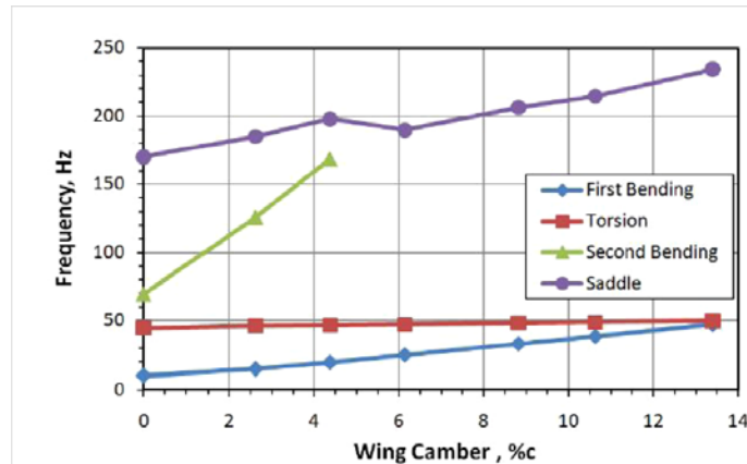
Figure 1.15: Effect of camber on \omega_n for the Manduca sexta Forewing [17].
