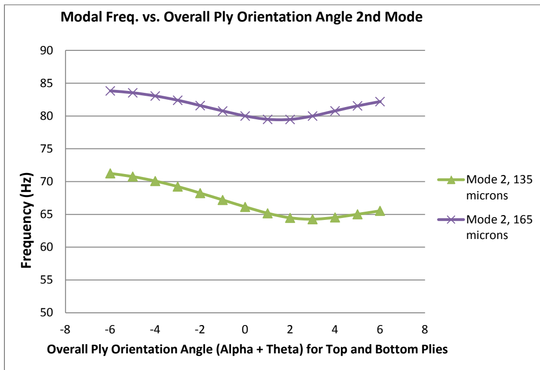
Figure 5.13: Comparison of the Second Mode For Varying Thicknesses.
