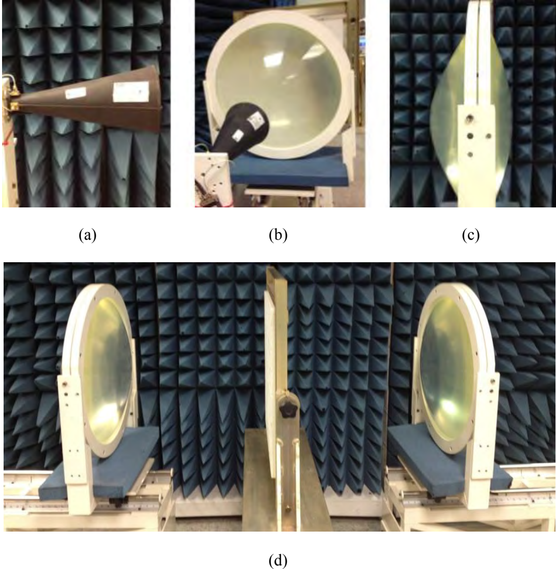
Figure 86. Pictures of the focus beam system setup for S-parameter measurements. (a) Picture of horn antenna. This can produce horizontal or vertical polarizations. (b) View from port 1. The horn antenna illuminates the back of the lens. (c) Picture of the port 1 compound lens. (d) Picture of center mount between the port 1 (left) and port 2 (right) lenses. Note the symmetrical spacing of the system.
