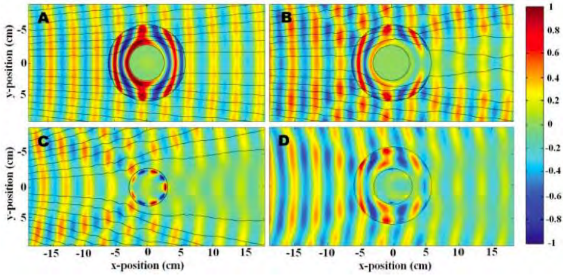
Figure 41. Simulated and measured steady-state electric field patterns at various instances in time in [55]. (a) Simulated field patterns for the exact metamaterial cloak. (b) Simulated field patterns for the cloak with reduced material properties. (c) Measured field patterns for the bare, conducting cylinder. (d) Measured field patterns for the cloaked conducting cylinder.
