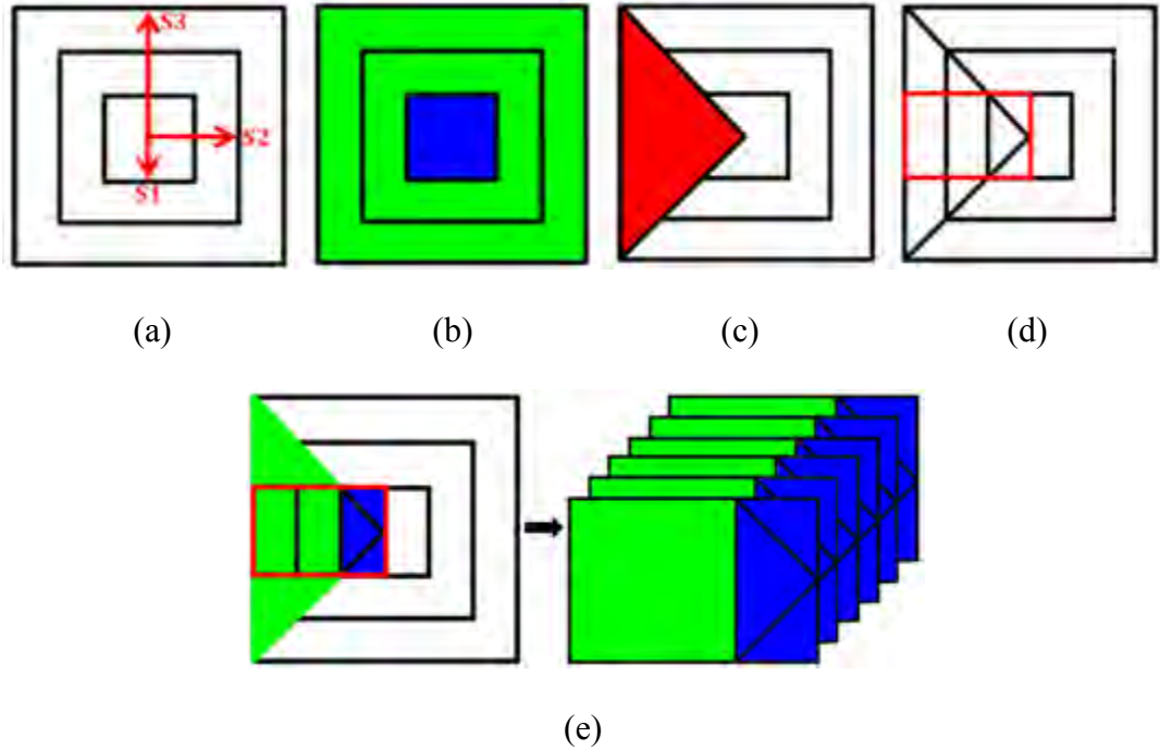
Figure 44. Basic design of the field concentrator. (a) Design was based on a design of three concentric squares of increasing half-width: S1 , S2 , and S3 . (b) Innermost region, colored blue, is used to compress the fields while the outer two squares provide the expansion. (c) Only one quadrant of the square design is manufactured. (d) Simplest manufacturable geometry from one quadrant is the rectangular board drawn with a red line. (e) Superposition of (b) and (d) show which areas of the manufactured design will be compression and which will be expansion. (f) Manufactured device is an array of parallel, stacked rectangular boards.
