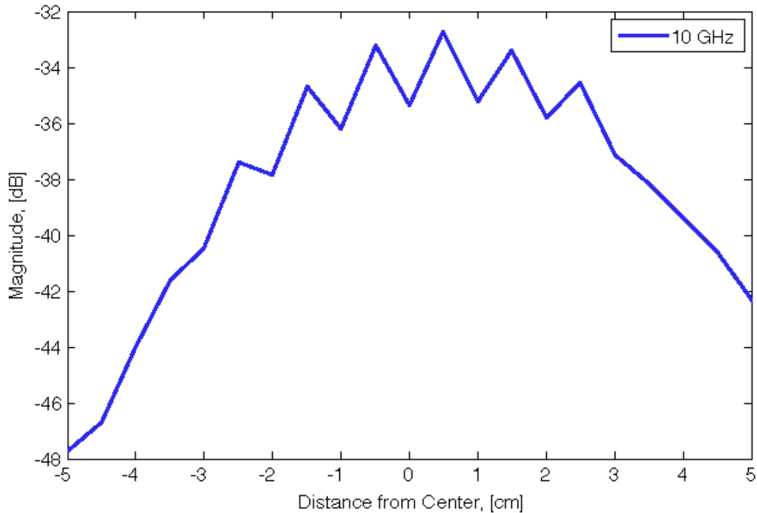
Figure 108. Plot of the transmission magnitude for a Gaussian, collimated 10 GHz signal in the middle of the center mount with the foam holder in place. The saw-tooth peak centered at the origin is indicative of constructive and deconstructive interference due to diffraction from the edges of the foam holder. The asymmetrical nature of the lobing with respect to the center of the foam holder indicates misalignment of likely both my probe and the foam holder with respect to the path of incident plane waves.
