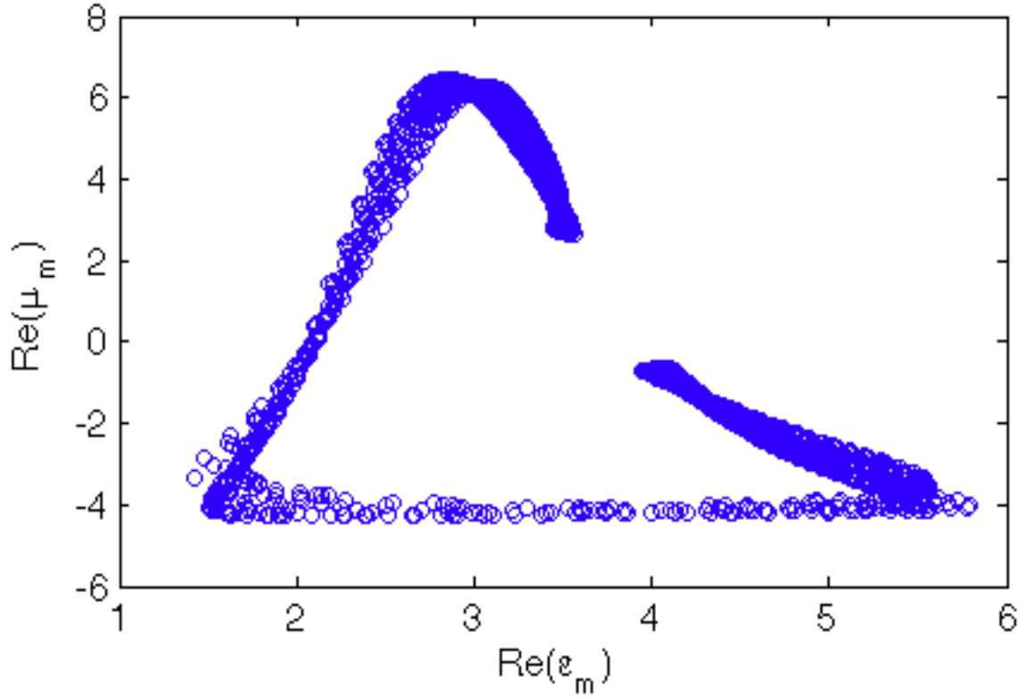
Figure 45. Plot of the real, achievable constitutive parameters for TLY-5.
