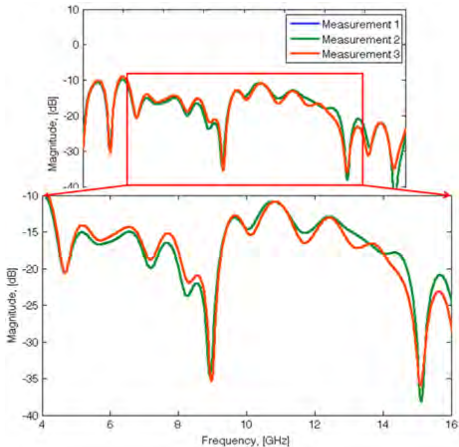
Figure 97. Plot of all three transmission magnitude measurements for the DUT evenly positioned in the foam holder. Plot data are smoothed and gated.
