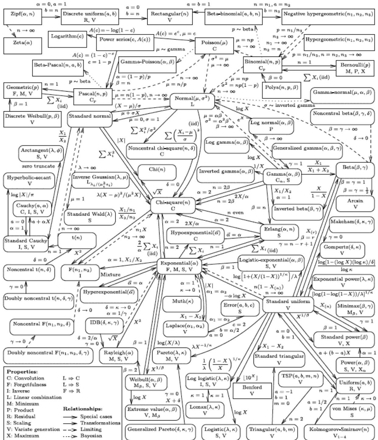
Figure 1: Univariate distribution relationships (Leemis and McQueston 2008)
