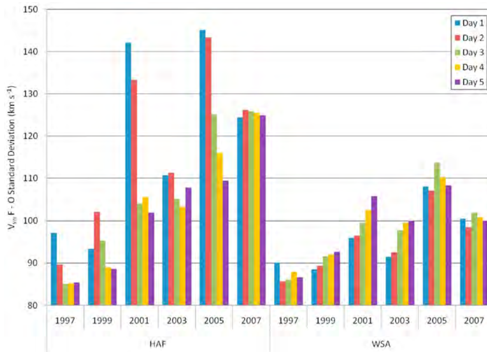
Figure 3. Same as Figure 1 except for F-O standard deviation.
