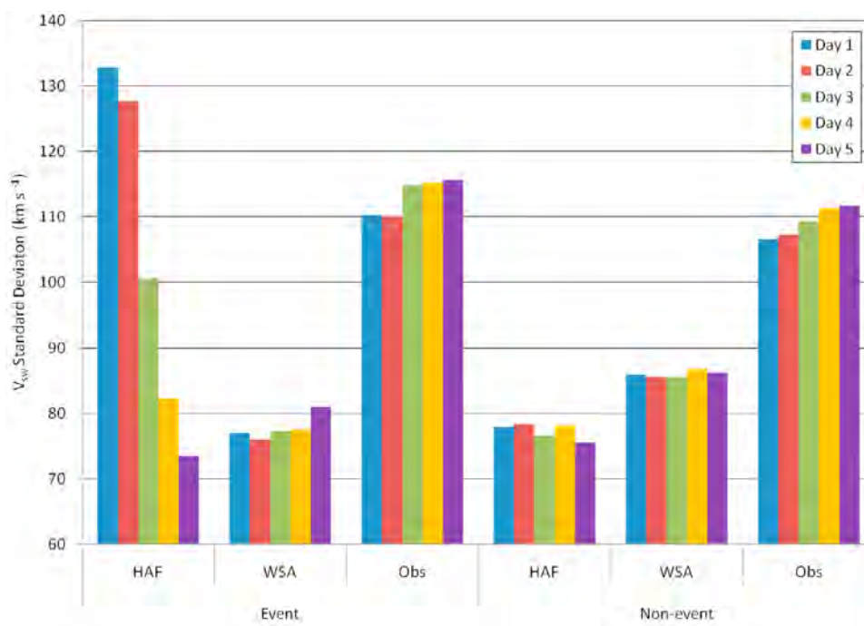
Figure 8. Standard deviation of HAF, WSA, and observed V_{sw} computed separately for event and nonevent forecasts over all study years by forecast day.
