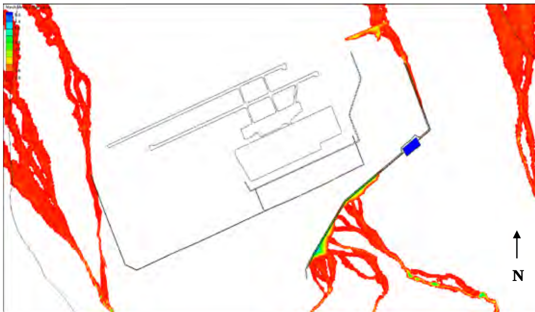
Figure 80. Alternative 3-C maximum flood inundation depth, m.
