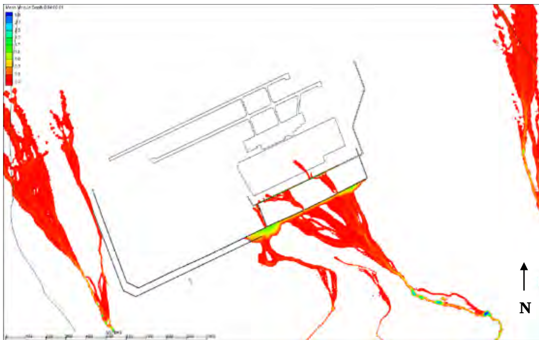
Figure 45. Alternative 1-B inundation depths, at 4 hours, m.
