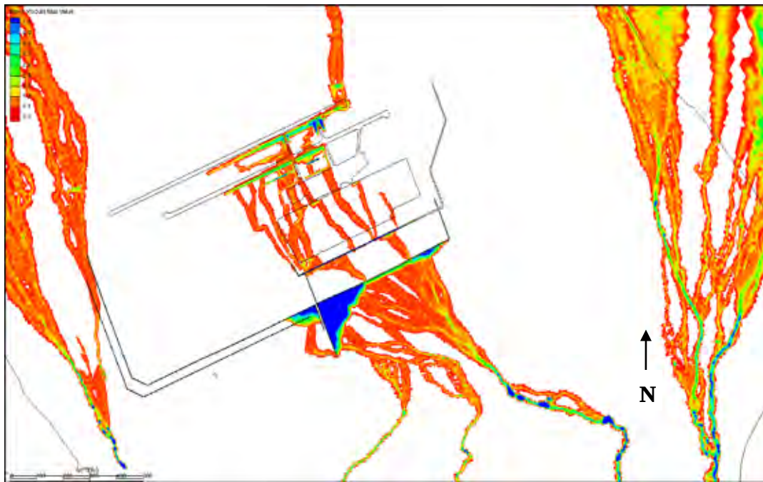
Figure 91. Maximum flood inundation depth, German alternative, m.
