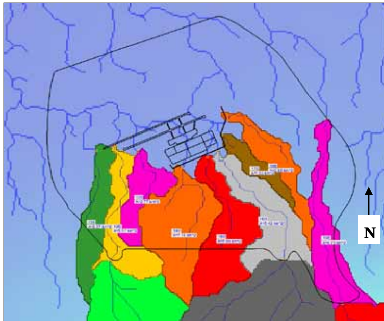
Figure 8. Interior to the domain contributing watersheds.
