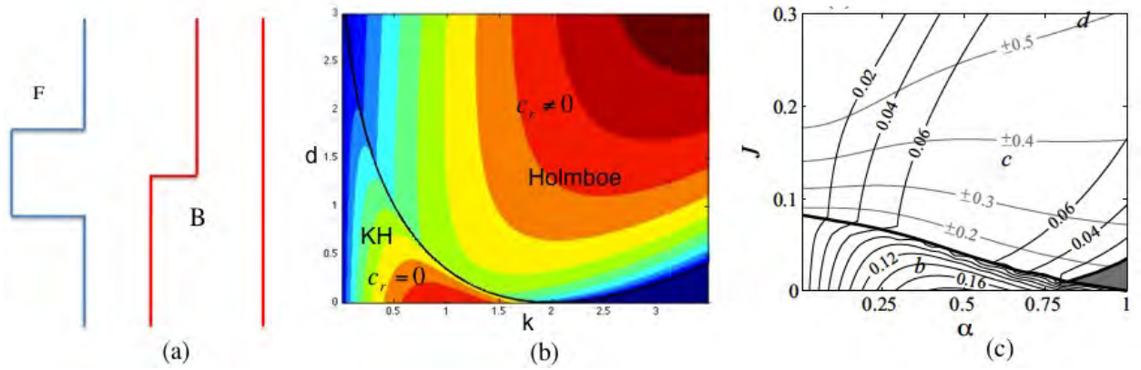
Figure 5: Holmboe instability. a) A broken-line profile, b) Contours of growth-rate ( c_i ) in d-k plane ( f = 2 ), c) Growth-rate contours in Ri-k plane from a complete linear stability calculations (Carpenter et al.[8])
