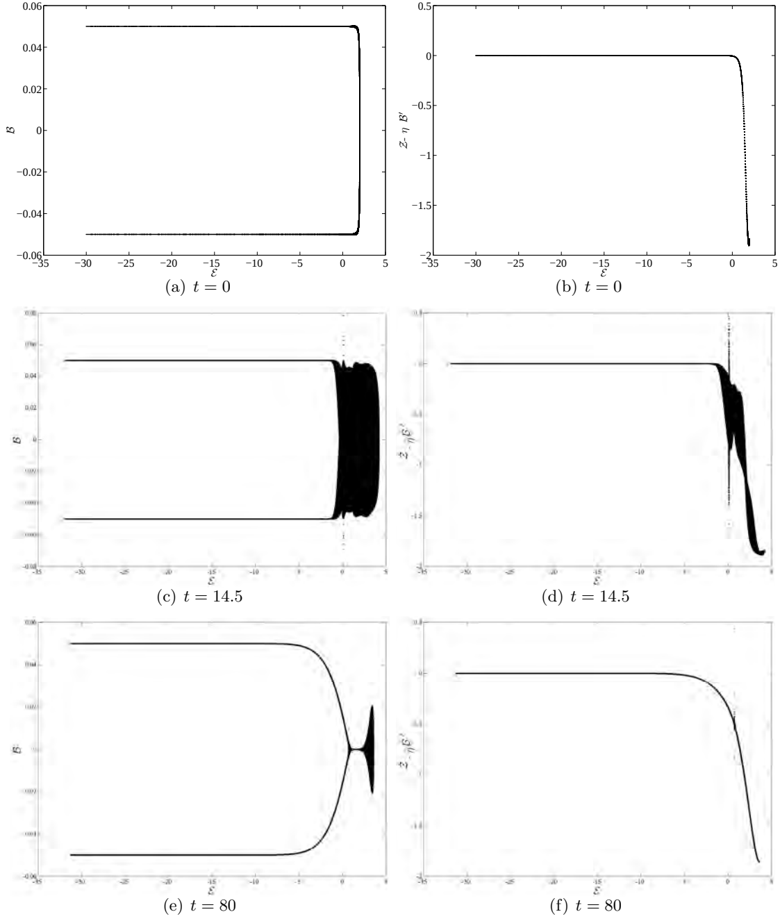
Figure 20: Nonlinear stationary state diagnostics for stratified KH instability. Time evolution of the dependence of B with \varepsilon is shown in (a), (c) and (e) and that of Z - \eta B' with \varepsilon in (b), (d) and (f).
