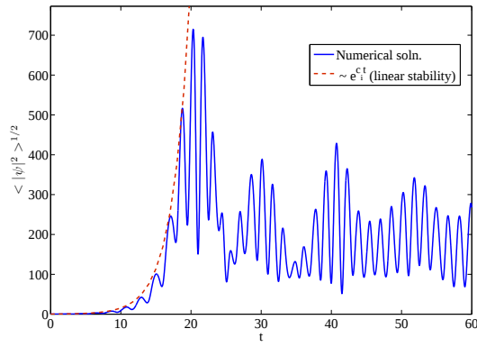
Figure 12: Evolution of disturbance amplitude for pure Holmboe instability. c_i = 0.4005
